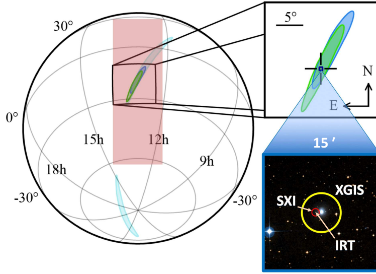
Fig. 1. The plot shows the THESEUS/SXI field of view ( \sim 110 \times 30 \text{ deg}^2 , pink rectangle) superimposed on the probability skymap of GW 170817 obtained with the two Advanced LIGO only (cyan) and with the addition of Advanced Virgo (green) (Abbott et al. 2017c). THESEUS not only will cover a large fraction of the sky (even those obtained with only two GW-detectors, e.g. cyan area), but will also localize the counterpart with uncertainty of the order of 5 arcmin with the XGIS and to less than 1 arcmin with SXI. The THESEUS location accuracy of GW events produced by NS-NS mergers can be as good as 1 arcsec in case of detection of the kilonova emission by the IRT. By the end of the 2020s, if ET will be a single detector, almost no directional information will be available for GW sources ( > 1000 \text{ deg}^2 for BNS at z > 0.3 , Zhao & Wen e.g. 2017), and a GRB-localising satellite will be essential to discover EM counterparts.
