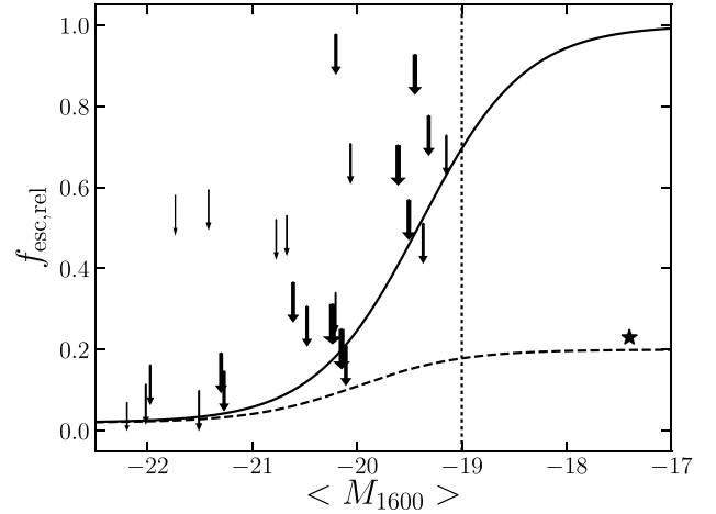
Figure 12. Relative escape fraction upper limits as a function of absolute magnitude. Solid line represents an estimated upper-limit envelope (equation 7). Dashed line shows the f_{\text{esc}}(M_{\text{UV}}) relation for which the modelling produces a background best matching with the data (see the text and Fig. 13, left-hand panel, right column). Shown is also the escape fraction upper limit measured by Amorín et al. (2014) for a single faint galaxy (star).
