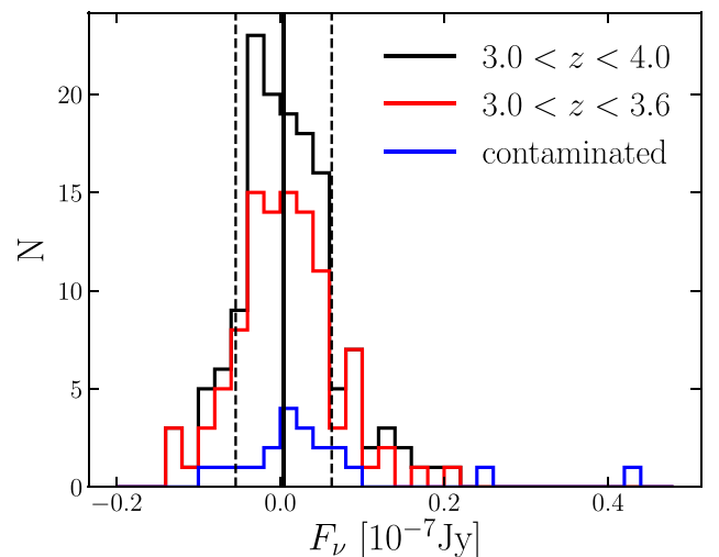
Figure 6. UVIS/ F_{336W} fluxes measured at the galaxy positions (see the text for details). Mean value and standard deviation are shown with full and dashed lines, respectively. These values are very similar for both 3 < z < 4 and 3 < z < 3.6 ranges. Emission may have potentially been detected with >3\sigma significance in four cases – see Fig. 7 for more details on their properties.
