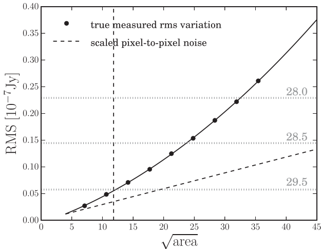
Figure 2. Measurement of the depth of the (30 mas pixel −1 ) drizzled image of the UVUDF field taken in UVIS/F336W filter (Rafelski et al. 2015). RMS is shown as a function of \sqrt{A} of the aperture with area A (in pixels). Horizontal dotted lines indicate the corresponding 1\sigma upper limits (in magnitudes). Dashed line: assuming uncorrelated noise, pixel-to-pixel variation ( \sigma_i ) is scaled to the desired aperture as \text{RMS} = \sigma_i \sqrt{A} . This results in a 1\sigma ( 5\sigma ) limiting magnitude in the 0.2 arcsec aperture of 30.0 (28.3) mag. Black circles: directly measured flux variations in circular apertures of different sizes. Full line is a polynomial fitted to the points and does not represent a physical model. This method results in a 1\sigma ( 5\sigma ) limiting magnitude of 29.5 (27.8) mag. Vertical dashed line corresponds to 0.2 arcsec aperture. Measurements are obtained using Monte Carlo simulations and only in regions of the image where no sources have been detected.
