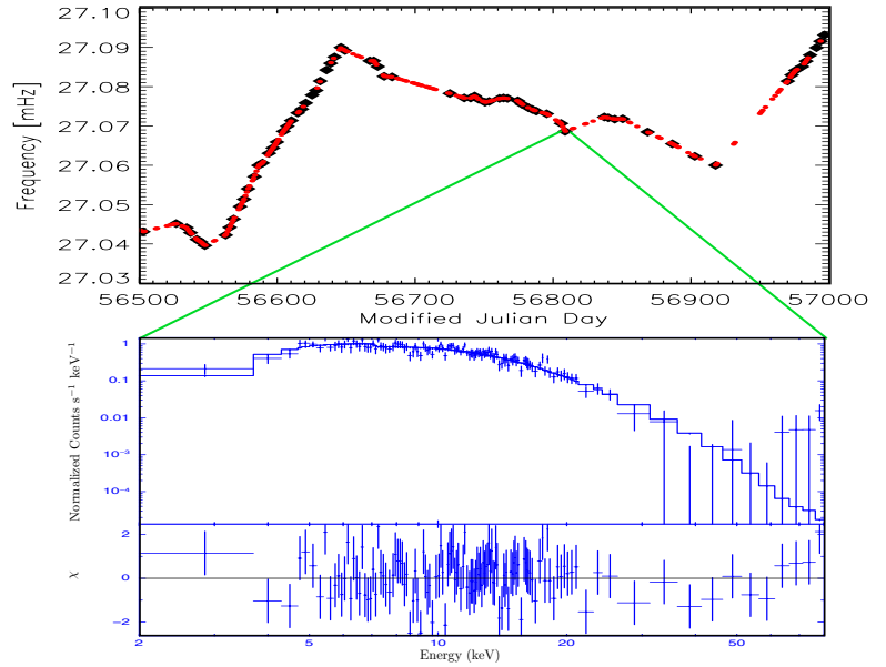
Figure 10: The frequency history from GBM pulsar monitoring (black diamonds) along with the simulated detections from the WFM (red disks). The frequencies were modeled from results by the Fermi/GBM and the source fluxes were taken from Swift/BAT. We used the source spectral model proposed by (Pradhan et al., 2014). An improved detection rate where the source dips below GBM’s sensitivity is due to WFM’s sensitivity below 8 keV. Compared to the GBM, pulsations are also detected earlier and with higher resolution by the WFM, enabling us to monitor the pulsed portion of the outburst during the critical onset stages of the event. The WFM will also be able to follow at any time the spectral evolution of the source in a wide energy band and with good resolution (as shown in the bottom panel).
