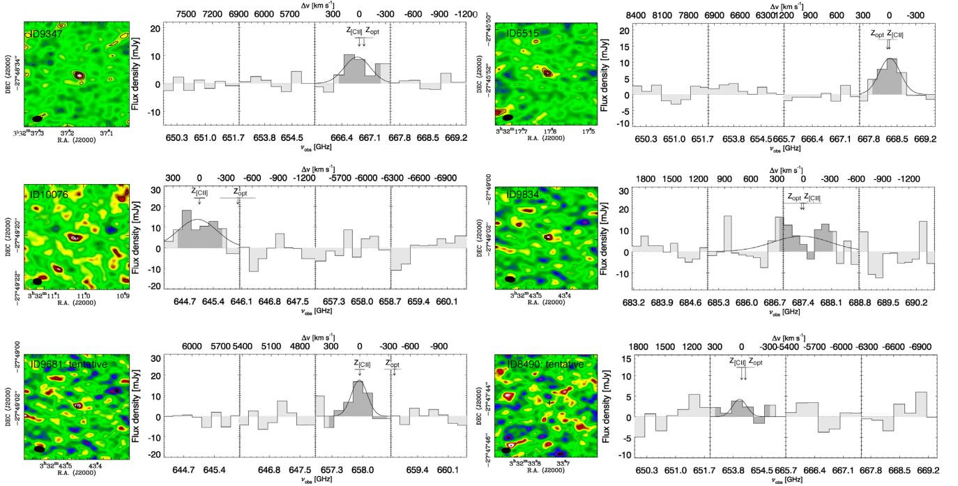
Figure 2. ALMA spectra of the [C II] detections of our sample. Left panels: ALMA 2D maps of the [C II] emission line. The black solid and dashed contours indicate respectively the positive and negative 3\sigma , 4\sigma , and 5\sigma levels. The beam is reported as the black filled ellipse. Each stamp has a size of 4'' \times 4'' . The black cross indicates the galaxy center, as estimated from the HST F160W imaging. Some tapering has been done for illustrative purposes, although we used the untapered maps for the analysis. Right panels: 1D spectra of the [C II] detected sources extracted using a PSF to maximize the S/N (notice that in this figure we did not scale the fluxes of the spectra extracted with PSF to match those obtained when using an exponential function with larger size as reported in Table 2). The dark grey shaded areas indicate the 1\sigma velocity range over which the flux has been measured. The frequencies corresponding to the optical and [C II] redshifts are marked with arrows. The horizontal bars indicate the 1\sigma uncertainty associated to the optical (light gray) and [C II] (dark gray) redshift estimate. For illustrative purposes we also report the Gaussian fit of the emission lines: it was not used to estimate the line fluxes, but only as an alternative estimate of the galaxies' redshift (Section 2.3).
