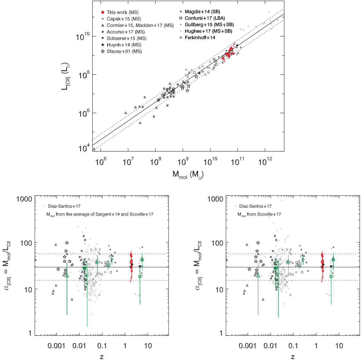
Figure 8. Correlation between the [C II] luminosity and the molecular gas mass. Top panel: L_{\text{CII}}-M_{\text{mol}} relation. The symbols are the same as reported in Fig. 6 caption, but we only show the samples with available M_{\text{mol}} estimates. In the legend we highlight the nature of the galaxies in each sample (e.g. MS, starburst, Ly break analogues). The fit of the data is reported (black solid line) together with the standard deviation (black dashed lines). Bottom panels: the [C II]-to- \text{H}_2 conversion factor ( \alpha_{\text{CII}} ) as a function of redshift. The average \alpha_{\text{CII}} for MS galaxies is reported (black solid line) together with the standard deviation (black dashed lines). The median and median absolute deviation of each sample are plotted (green large symbols). The difference between the left- and right-hand panels concerns how the molecular gas mass was estimated for the sample of local galaxies from Diaz-Santos et al. (2017, light gray crosses). Since CO observations for this sample are not available, we estimated M_{\text{mol}} , given the sSFR of each source, considering the relation between the depletion time and sSFR of galaxies. In the left-hand panel we report the estimates obtained by averaging the trend reported by Sargent et al. (2014) and Scoville et al. (2017), whereas in the right-hand panel we report the estimates obtained considering the trend by Scoville et al. (2017) only (see Section 3.3 for a more detailed discussion).
