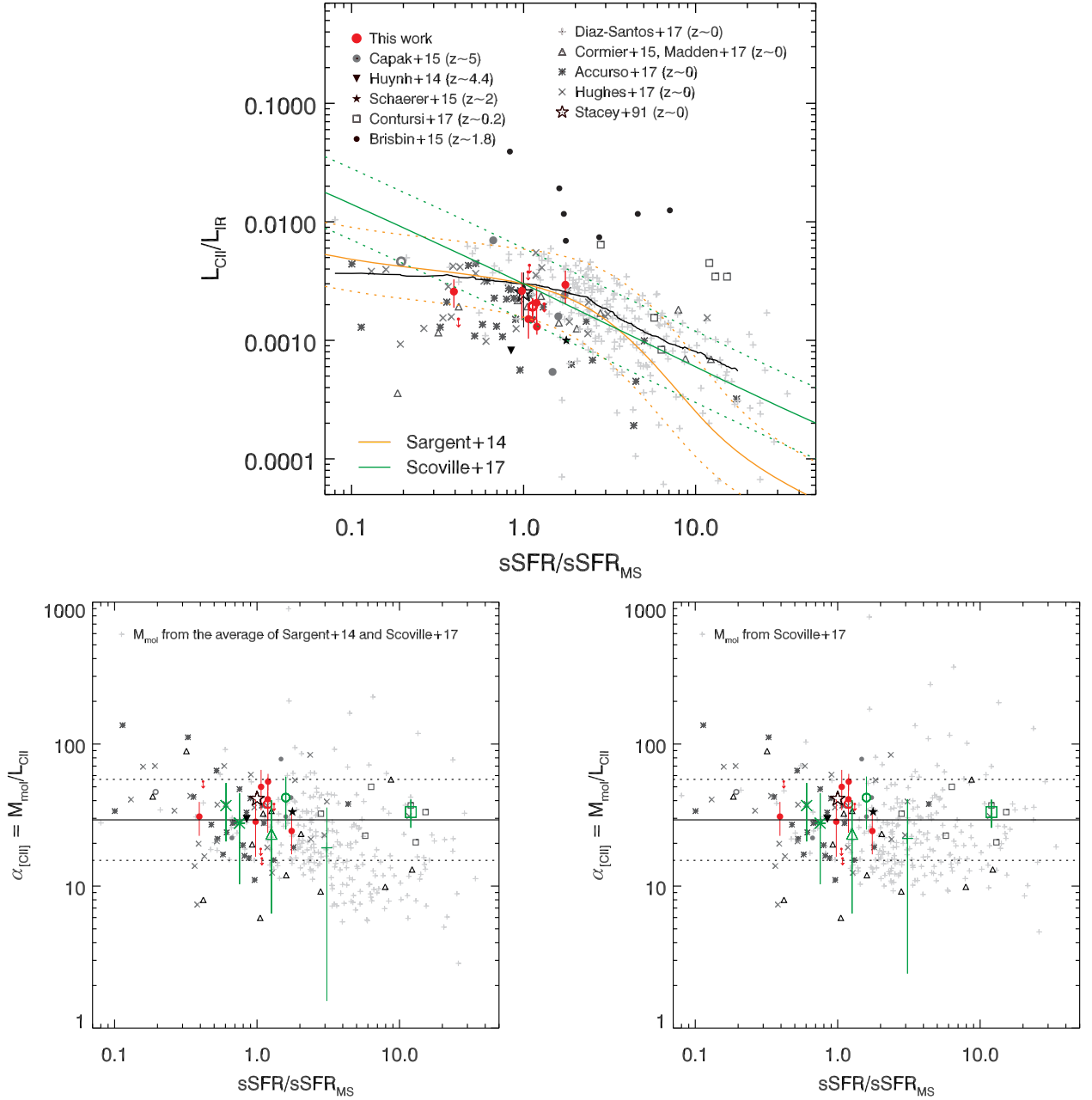
Figure 9. Correlation between the [C II] luminosity and galaxies’ distance from the MS. Top panel: [C II]-to-IR luminosity ratio as a function of the galaxy distance from the MS. The symbols are the same as reported in the Fig. 6 caption. Additionally, we include the average of the local star-forming galaxies from Stacey et al. (1991, cyan star). In particular, the sources by Brisbin et al. (2015) might be lensed, but the magnification factors are unknown and therefore we plot the observed values. We also show the running mean computed considering all the plotted datapoints a part from the sample from Contursi et al. (2017, black solid line). Finally we report the model by Sargent et al. (2014, yellow curve) and Scoville et al. (2017, green curve), showing the trend of the depletion time as a function of the sSFR, renormalized to match the observed L_{\text{[C II]}}/L_{\text{IR}} ratios (the standard deviations of the models are marked as dashed curves). Bottom panels: dependence of \alpha_{\text{[C II]}} from galaxies’ distance from the MS. The difference between the left- and right-hand panels concerns how the molecular gas mass was estimated for the sample of local galaxies from Diaz-Santos et al. (2017, light gray crosses). Since CO observations for this sample are not available, we estimated M_{\text{mol}} , given the sSFR of each source, considering the relation between the depletion time and sSFR of galaxies. In the left-hand panel we report the estimates obtained by averaging the trend reported by Sargent et al. (2014) and Scoville et al. (2017), whereas in the right-hand panel we report the estimates obtained considering the trend by Scoville et al. (2017) only (see Section 3.3 for a more detailed discussion).
