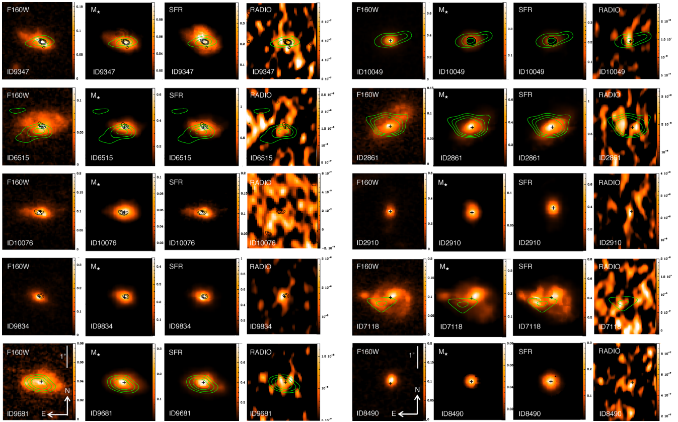
Figure 1. HST and ALMA observations of our sample galaxies. For each source we show the HST /WFC3 image taken with the F160W filter, the stellar mass map, the SFR map, and the radio observations taken with VLA. The overplotted black contours, when present, show the >3\sigma [C II] emission. The green contours indicate the >3\sigma 850 \mu\text{m} continuum. The color scale in all panels is linear and it is chosen to show galaxies' features at best. The units of the color bars are the following: counts \text{s}^{-1} for F160W, 10^9 M_{\odot} for the stellar mass maps, M_{\odot} \text{yr}^{-1} for the SFR maps, and Jy for the radio.
