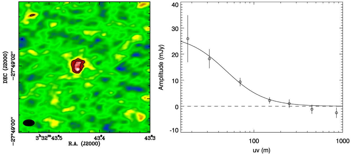
Figure 4. Stacking of the four secure [C II] detections of our sample. Left-hand panel: image obtained aligning the four galaxies at their HST peak positions and stacking their visibilities. From 3\sigma and 4\sigma contours are shown. Right-hand panel: signal amplitude as a function of the uv distance (namely the baseline length). We fitted the data with an exponential model (black curve). A similar fit is obtained when fitting the data with a gaussian model with FWHM \sim 0.6 arcsec.
