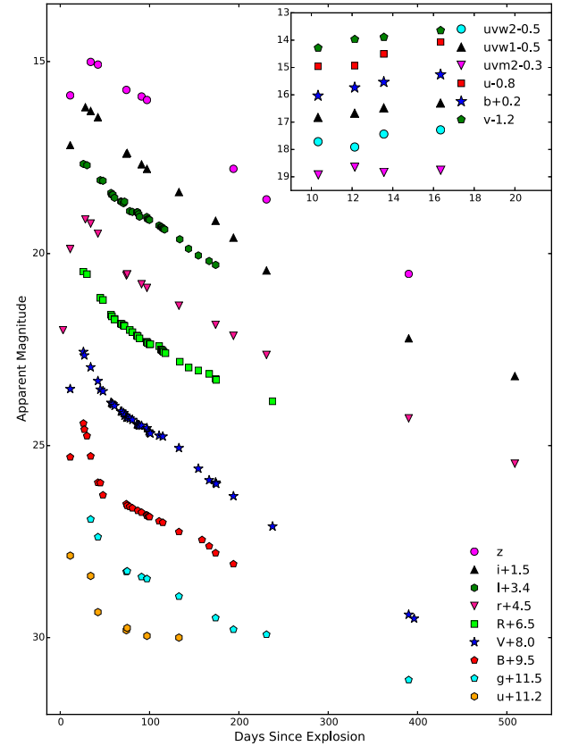
Figure 3. BVRI/ugriz light-curve evolution of SN 2015as. Inset plot shows the light-curve evolution of the UVOT filters. Explosion epoch is taken as 2015 November 6 (JD = 2457332.5). The light curves are shifted arbitrarily for clarity.
