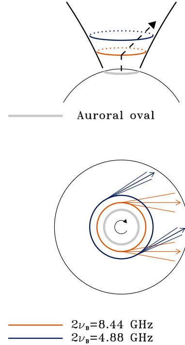
Figure 7. Top panel, side view of the auroral cavity that radiates at 4.88 and 8.44 GHz (assuming B_p = 3000 [Gauss]). The footprint at the stellar surface is also pictured (auroral oval). In the bottom panel is shown the top view of the auroral cavity. The auroral beam pattern at the two analysed frequencies is shown. The corresponding bended magnetic field line is schematically pictured in the top panel (dashed line).
