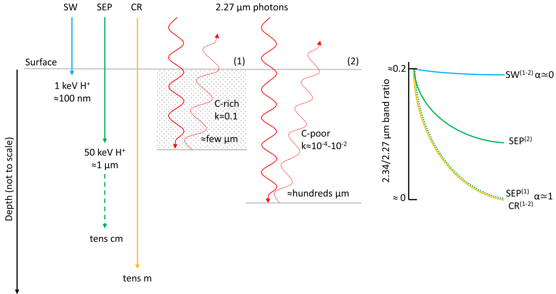
Figure 4. Penetration depths of SW, SEP, and CR. For SW and SEP we show 1 keV H^+ and 50 keV H^+ , respectively, the main populations in terms of energy and flux. Red arrows represent incident (solid) and reflected (dotted) 2.27 \mu m photons on a surface rich in amorphous carbon (C-rich) or rich in frozen volatiles (C-poor). The right part of the figure shows expected 2.34/2.27 ratios after irradiation by SW, SEP, and CR according to the IR-sampled thickness and the expected values of \alpha .
