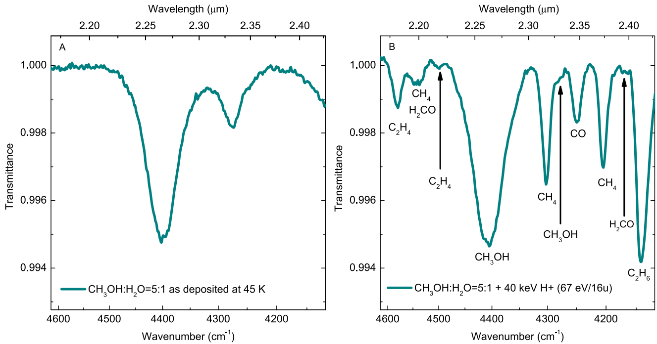
Figure 3. Comparison between the spectra of \text{CH}_3\text{OH}:\text{H}_2\text{O} = 5:1 mixture before (panel (A)) and after irradiation with 40 keV \text{H}^+ at 45 K (panel (B)). Labels indicate the compounds responsible for the absorptions.
