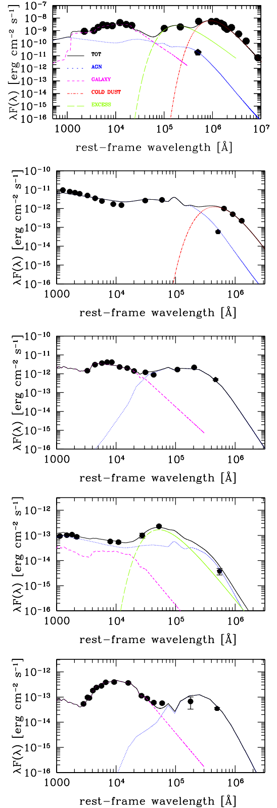
Fig. 3. Example of SED fitting results. From top to bottom: one type 2 source from the Swift sample, one type 1 from the X-WISSH sample, one type 2 from the ASCA sample, one type 1 from the XXL sample and one type 2 from the COSMOS sample. The AGN, galaxy, cold dust and excess emission components are shown in different colors and line types (as stated in the legend of the first figure in the top panel). Black circles are the photometric points of the source. The virtual AGN pivotal photometric point at 50 \mu\text{m} , derived from the hard X-ray data, is shown as the black pentagon (see text for details).
