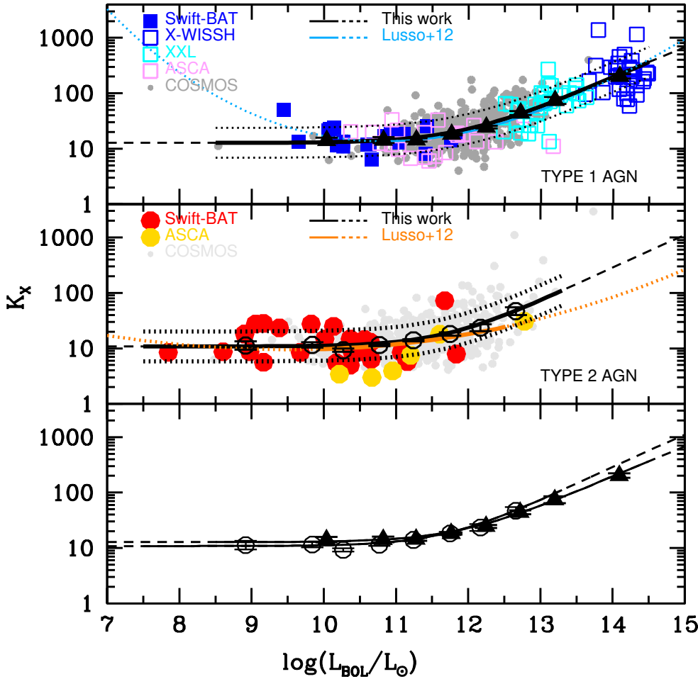
Fig. 4. Hard X-ray bolometric correction in the 2–10 keV band as a function of the bolometric luminosity for type 1 (upper panel) and type 2 (central panel) AGN. Symbols are as in the legend. Black filled triangles and open circles show the average values for type 1 and type 2 sources, respectively (directly compared in the lower panel), in bins of bolometric luminosity. The black solid and dashed lines show our best-fit relations and their extrapolations according to Eq. (2).
