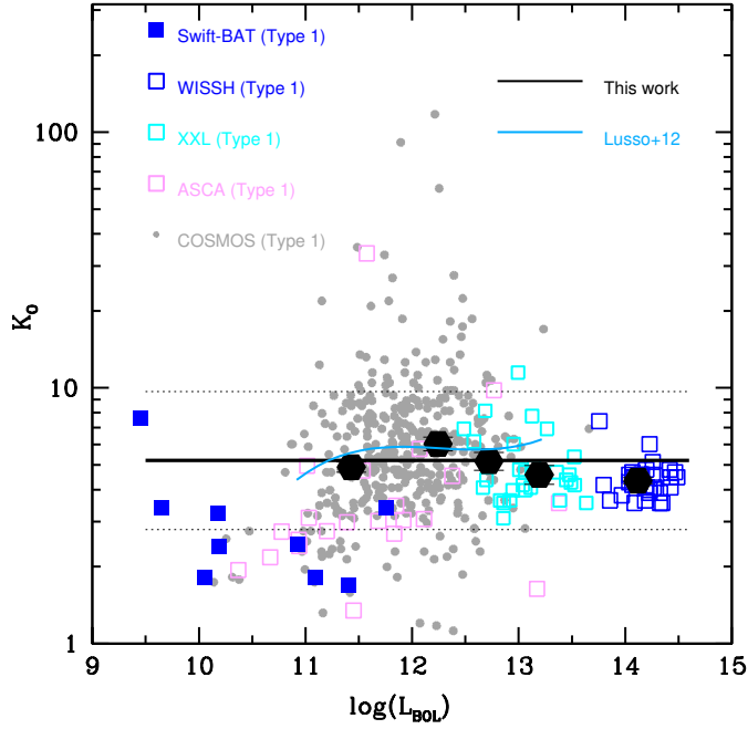
Fig. 7. Optical bolometric correction computed at 4400 \text{ \AA} for type 1 sources. The black solid line is our best-fit solution. See text and Table 2 for details.
