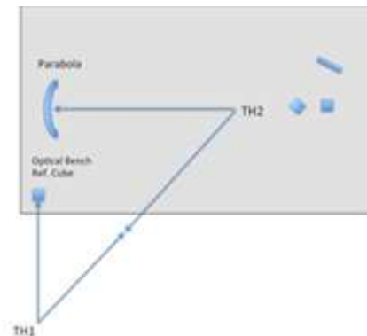
Figure 4. Schematics of the characterization of the OAP collimated beam direction in the GOBRS. The optical elements and the theodolites placements are shown.
