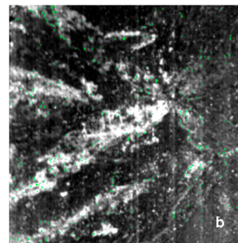
Figure 16. (a) Comparison between the spectral profile of pixel x74 y175 in bright region of sample B and the spectral signature of serpentine 1 from USGS library; (b) mapping of serpentine 1 spectrum on the whole bright area (green pixels).
