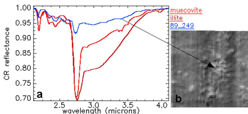
Figure 8. (a) Continuum removed spectral comparison between muscovite, illite, and pixel x89y249 of area A1 figure. (b) Pixel size is 38 \times 38 \mu\text{m} .
