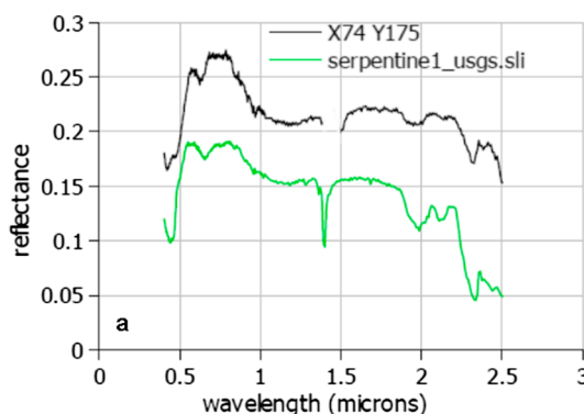
Figure 16. (a) Comparison between the spectral profile of pixel x74 y175 in bright region of sample B and the spectral signature of serpentine 1 from USGS library; (b) mapping of serpentine 1 spectrum on the whole bright area (green pixels).
