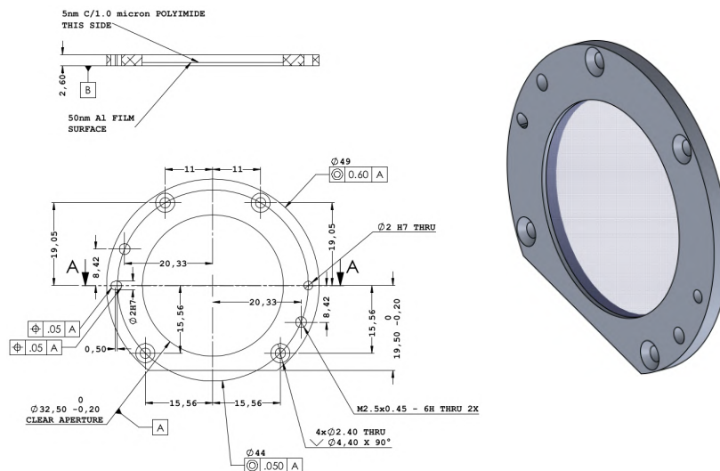
Figure 1: Drawing of the IXPE DU-FM ions-UV Filter. (All dimensions are in millimeters.)
