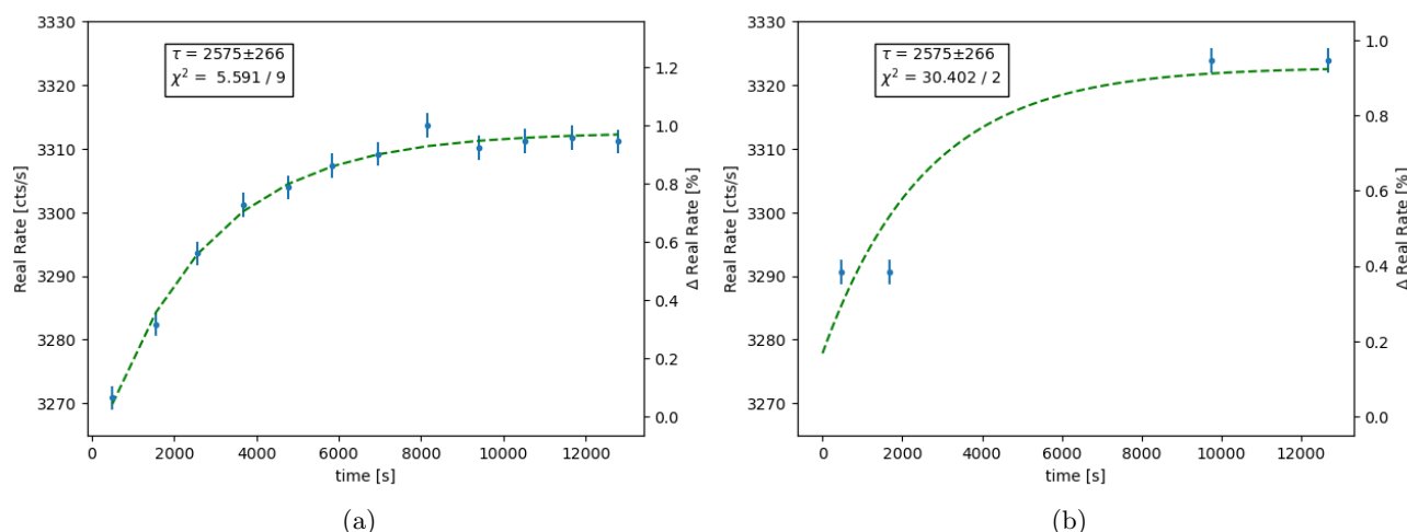
Figure 11: (a) Series of measurements obtained at 6.4 keV by collecting the same number of counts of the acquisition with the ions-UV filters ( 3 \cdot 10^6 counts) and a time interval of 2 minutes during which the X-ray source is turned off. They are fitted with an exponential function to obtain the time constant. (b) Reference measurements acquired in between the acquisitions with some ions-UV filters collecting the same number of counts ( 3 \cdot 10^6 counts). The fit function is an exponential function with time constant \tau that obtained by the previous fit.
