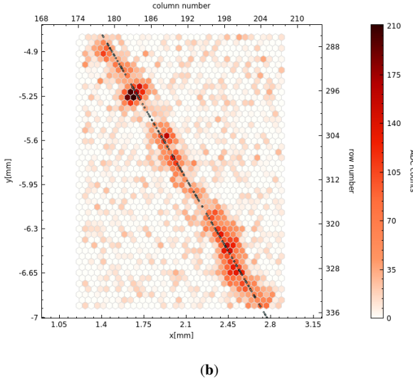
Figure 3: Imaging of tracks with random electronic noises from the simulation. The dots represent the energy deposit 2D positions inside the gas recorded by Geant4. (a): a track from a \text{Fe}^{55} decay X-ray photon and dashed line is the photoelectron eject direction. (b): a track from an energetic cosmic ray proton.
