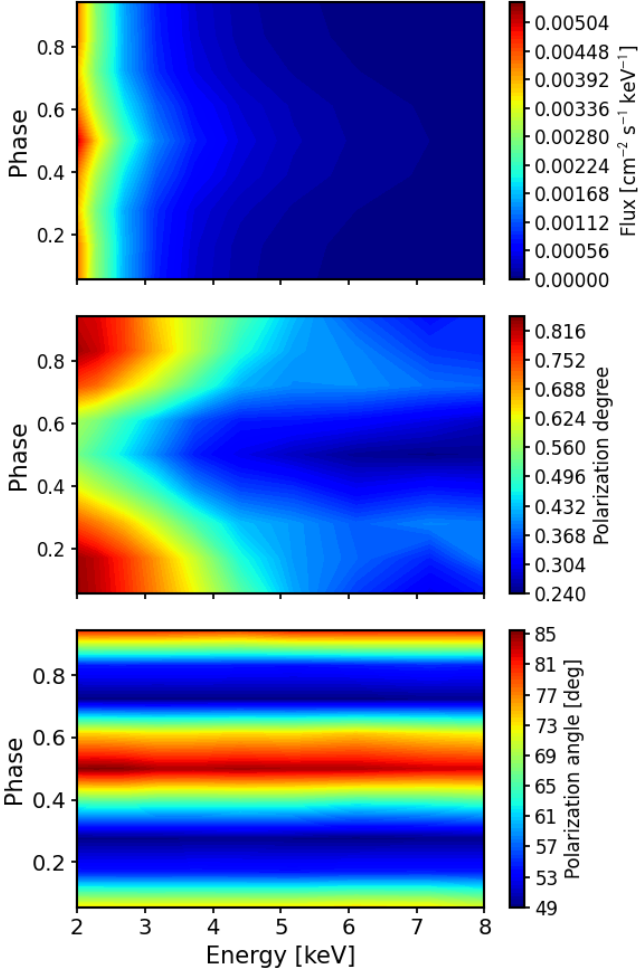
Figure 11: 1RXS J1708 source model ([23]). From the top to the bottom: source flux, polarization degree and polarization angle as functions of energy and phase.
