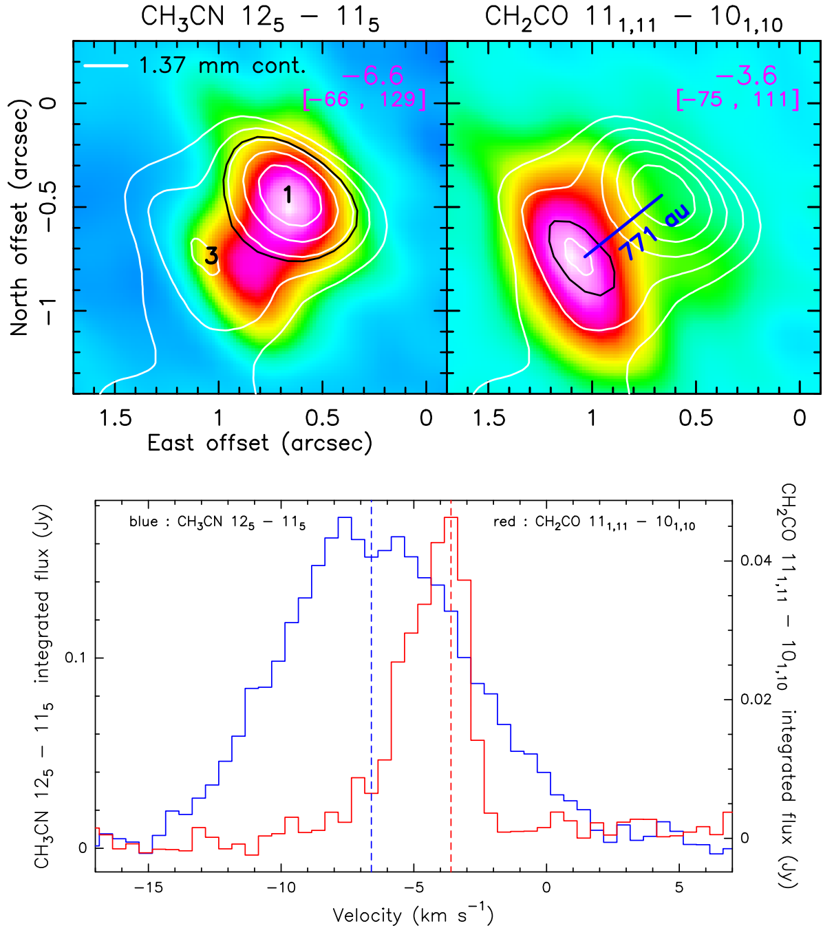
Fig. 8. NOEMA data. Upper panels: the color maps reproduce the emission of the CH 3 CN J_K = 12_5 - 11_5 (left) and CH 2 CO J_{K_a, K_c} = 11_{1,11} - 10_{1,10} (right) lines. In the upper right corner of the panel, the channel V_{\text{LSR}} (in kilometer per second) and the range of plotted values (in millijansky per beam) are reported. The white contours reproduce the 1.37 mm continuum, with the same levels as in Fig. 7: the positions of the two nearby 1.37 mm peaks are denoted using the same labels as in Beuther et al. (2018, see Table 5), namely, 1 and 3 for the primary and secondary peak, respectively. Right panel: the blue segment connects the two peaks. In the two panels, the black contours delimit the integration areas used to produce the spectra toward cores 1 and 3, presented in the lower panel. Lower panel: spectra of the CH 3 CN J_K = 12_5 - 11_5 line toward core 1 (blue histogram) and the CH 2 CO J_{K_a, K_c} = 11_{1,11} - 10_{1,10} line toward core 3 (red histogram). The flux scales for the CH 3 CN and CH 2 CO spectra are reported on the left and right, vertical axes, respectively. The blue and red dashed vertical lines indicate the approximate V_{\text{LSR}} of the cores 1 and 3, respectively.
