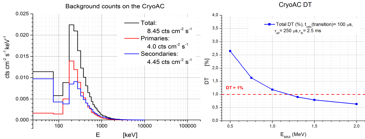
Figure 3. Left – Distribution of the expected energies deposited in the CryoAC absorber (500 um thick Silicon). Right - Expected DT vs the E_{\max} for \tau_{\text{th}} = 2.5 \text{ ms} and veto time in transition regime ( t_{\text{veto}} ) equal to the pulse peaking time (Color figure online).
