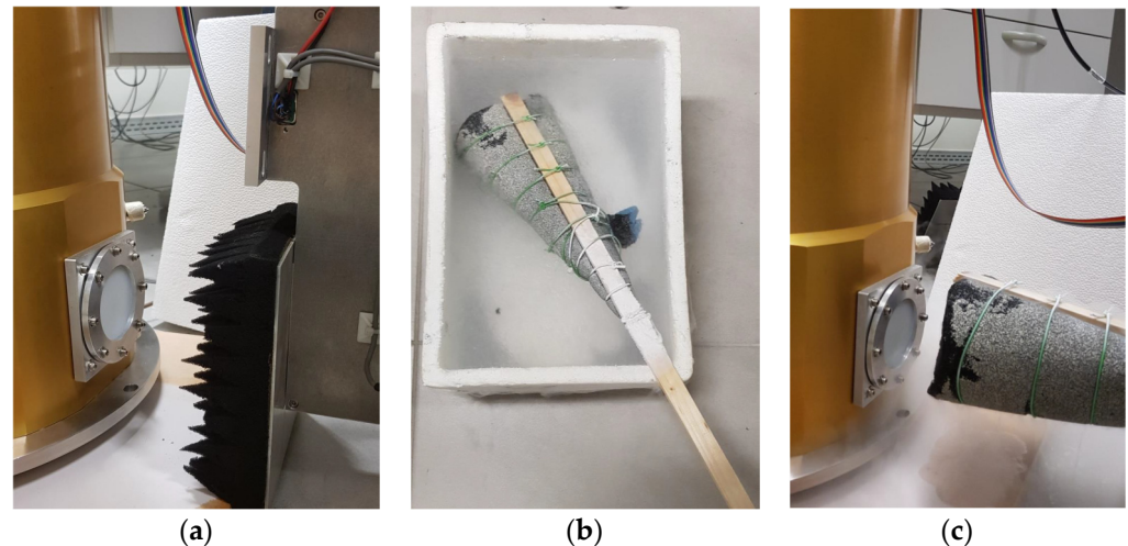
Figure 13. (a) Room temperature load placed in front of the HDPE system and the feed of the receiver. (b) Absorbing panel immersed in a container filled with liquid nitrogen. (c) Cold load placed in front of the HDPE system and the feed of the receiver.
