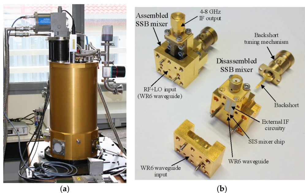
Figure 2. (a) Photo of the ex-PdBI receiver mounted on a laboratory test bench. (b) Photo of the single side band (SSB) superconductor–insulator–superconductor (SIS) mixer.
