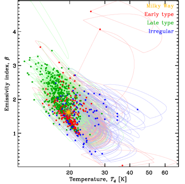
Fig. E.1. Modified black body results. The SUEs show the relation between the temperature, T_d , and the emissivity index, \beta , derived from the \beta -free MBB run presented in Sect. 3.3.2 . Galaxies are color-coded according to their type ( cf. Sect. 3.3.2 ). The diffuse ISM of the Milky Way ( T_d^{\text{MW}} = 20 \text{ K} , \beta_{\text{MW}} = 1.6 ; Planck Collaboration et al. 2014 ) is displayed as a yellow star.
