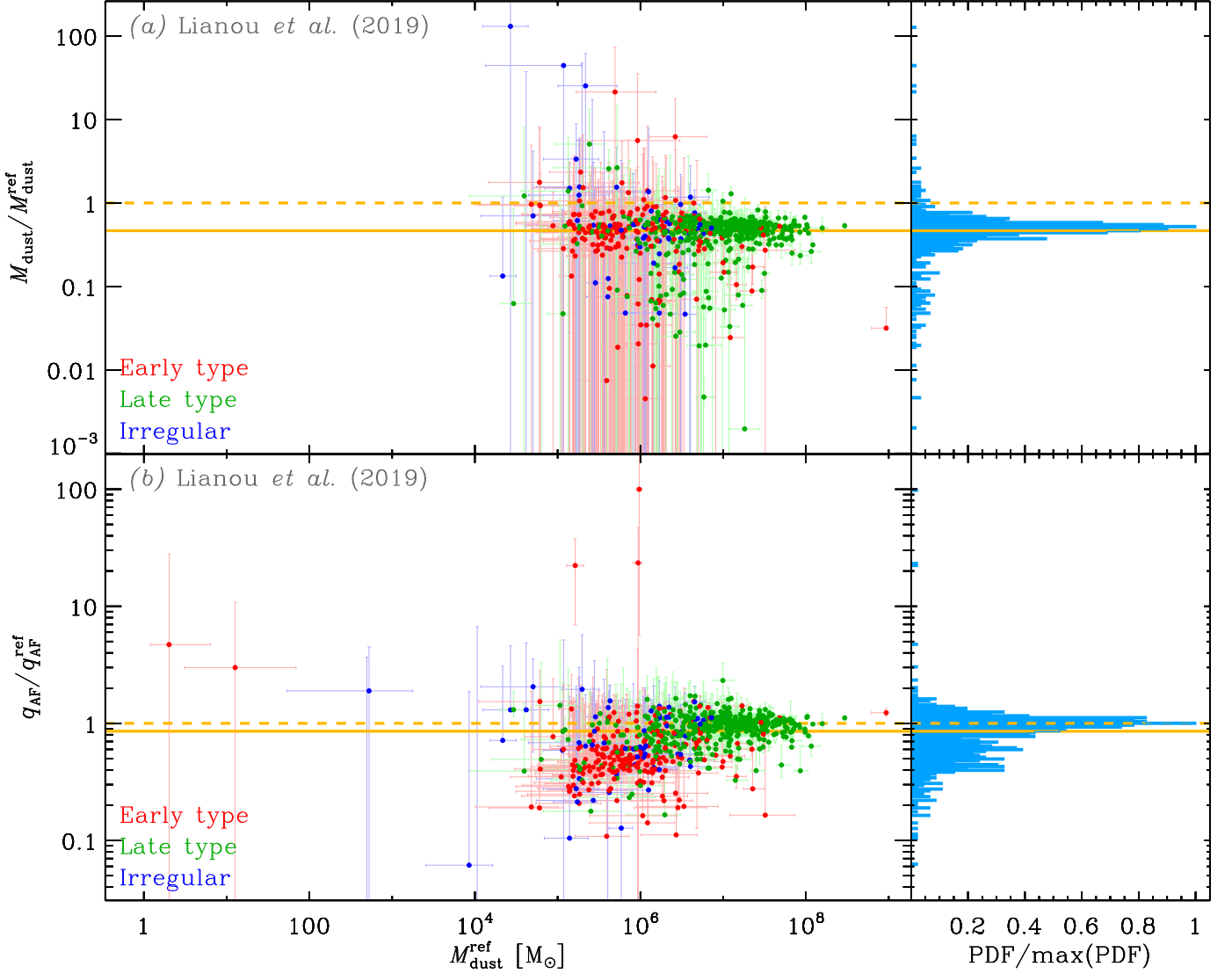
Fig. 7. Comparison to Lianou et al. (2019). Same conventions as Fig. 4.
