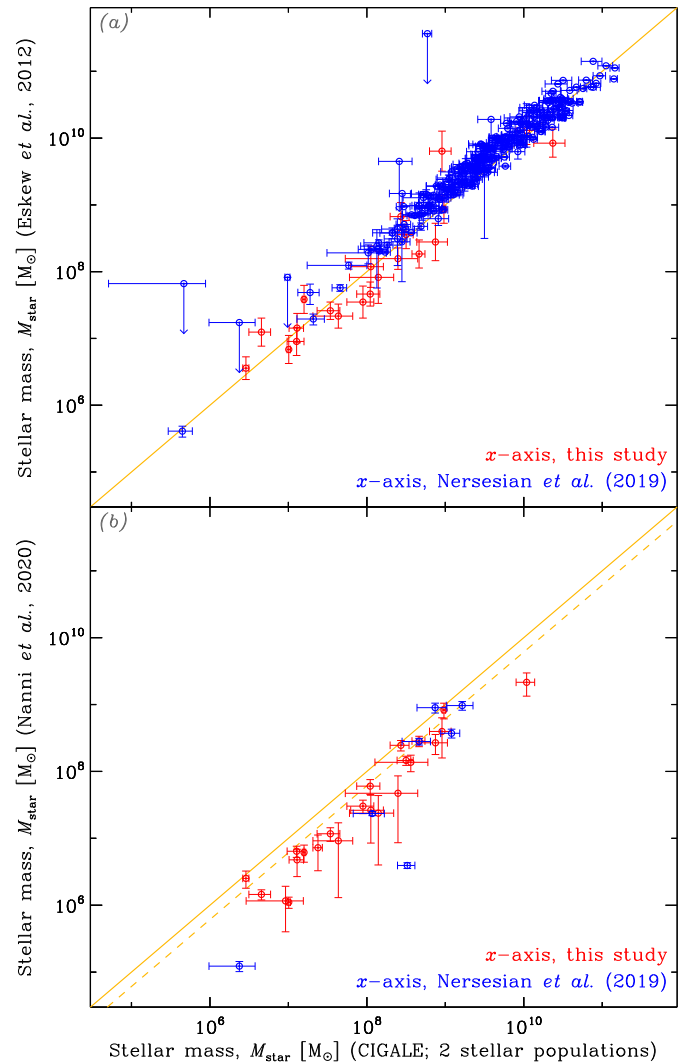
Fig. B.2. Comparison of stellar mass estimators. Panel (a) compares the CIGALE estimates of M_* , using two stellar populations ( x -axis), with the Eskew et al. (2012, y -axis) empirical approximation, both assuming a Salpeter (1955) IMF. Panel (b) compares the same x -axis as panel (a) to the CIGALE estimates, using a single stellar population and a Chabrier (2003) IMF, by N20. In both panels, the blue symbols correspond to the values presented in Nersesian et al. (2019), and the red symbols correspond to the values estimated for this study, with the same CIGALE settings. The solid yellow line represents the 1:1 relation. The dashed yellow line in panel (b) represents the 1:0.61 relation that accounts for the difference in IMFs.
