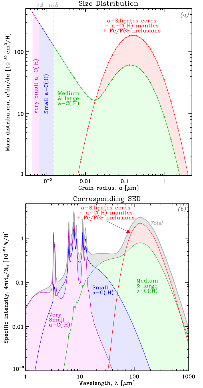
Fig. 1. Parametrization of the THEMIS model. Panel (a) shows the size distribution of the two main components of THEMIS: amorphous carbons and silicates. We show how we divide the a-C(:H) size distribution into three independent components. Panel (b) shows the SED corresponding to each component (same color code as panel a). The SED is shown for the ISRF of the solar neighborhood (Mathis et al. 1983).
