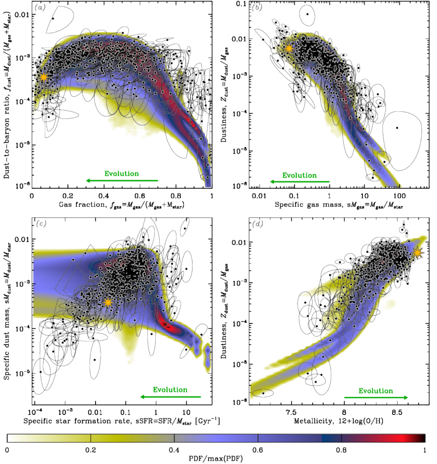
Fig. 14. Fitted dust evolution tracks, assuming a Salpeter (1955) IMF. The four panels represent the same quantities as Fig. 8 . The black SUEs represent the 556 galaxies of our subsample. The yellow star is the Milky Way. The colored density contours represent the posterior PDF of dust evolution tracks, marginalizing over the individual SFH of each galaxy.
