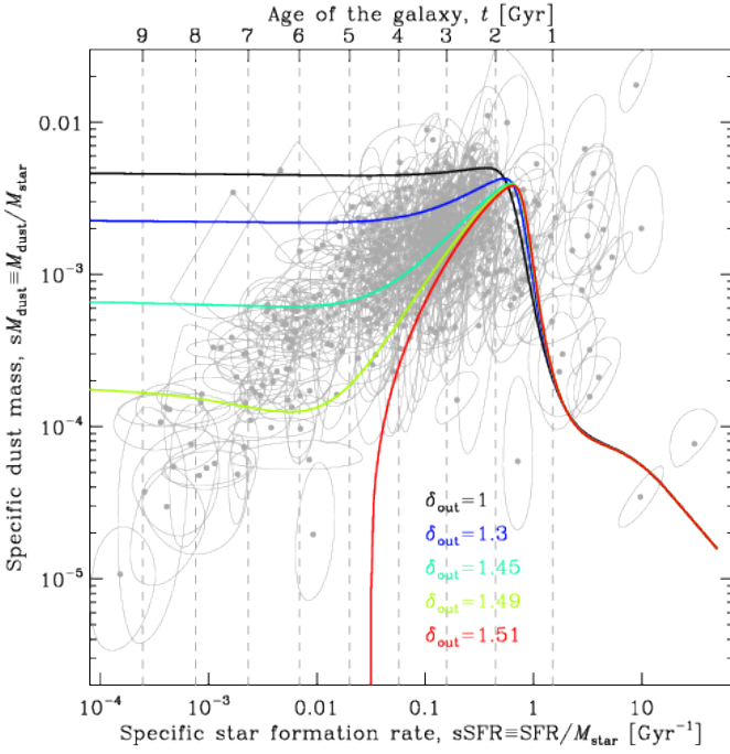
Fig. 15. Effect of outflow on the sM_{\text{dust}} - s\text{SFR} relation. The data is identical to panel (c) of Fig. 14. The colored lines represent our dust evolution model. We have fixed all the parameters close to their maximum a posteriori values, except the outflow rate, \delta_{\text{out}}: \tau_{\text{SFH}} = 0.8 Gyr, \psi_0 = 40 M_{\odot}/\text{yr} , \delta_{\text{in}} = 1.0 , \delta_{\text{SN}} = 0.01 , \epsilon_{\text{grow}} = 4500 and m_{\text{gas}}^{\text{dest}} = 1200 M_{\odot}/\text{SN} . The different lines correspond to different values of \delta_{\text{out}} . The top axis displays the age of the galaxy corresponding to the particular SFH of the model run. We have used a Salpeter (1955) IMF.
