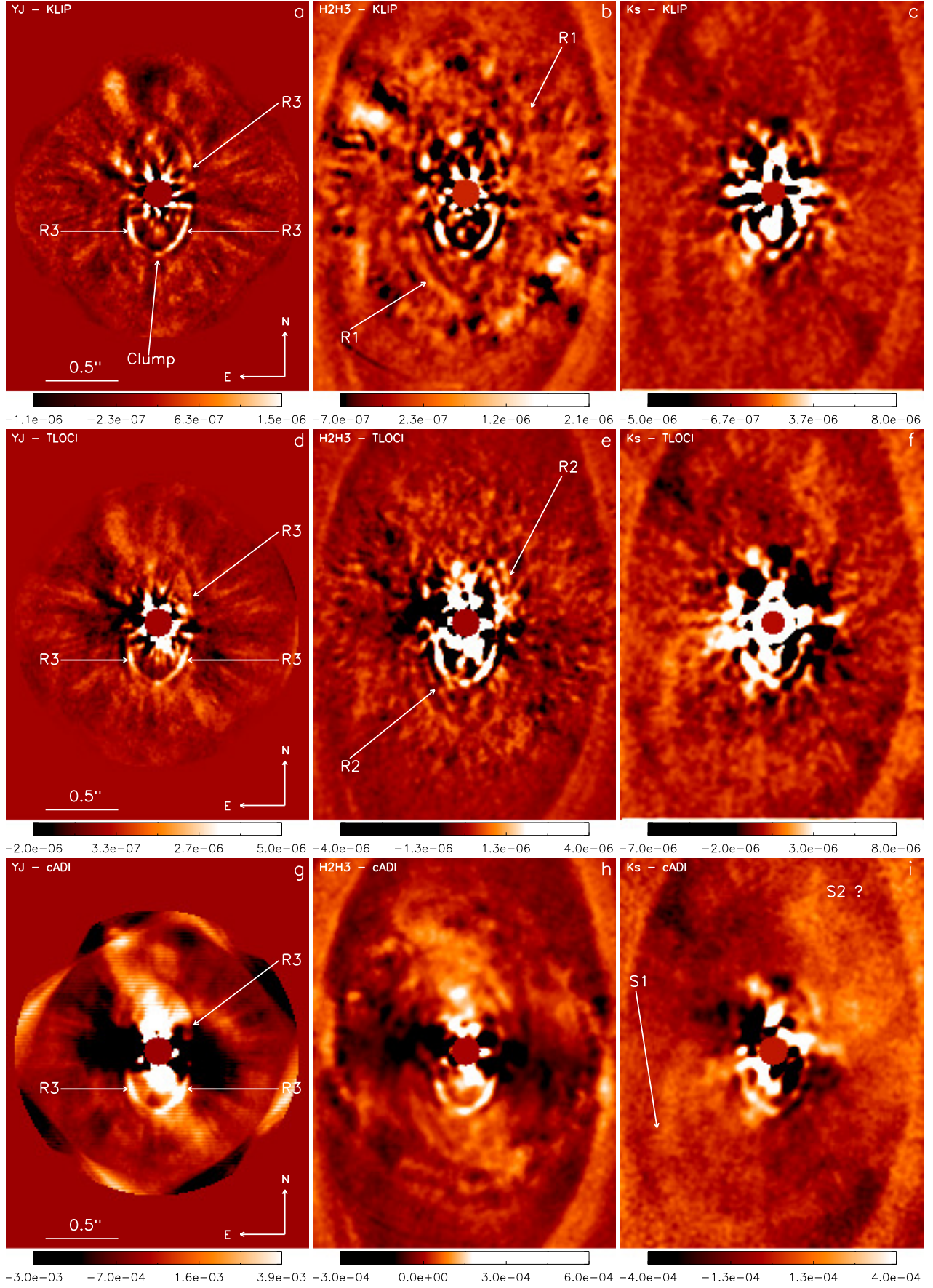
Fig. B.2. Images of the central part of the system in YJ (left column), H2H3 (middle column), and Ks (right column) bands with three different post-processing: KLIP (top row), TLOCI (middle row), and cADI (bottom row). The cADI images are multiplied by r to improve the visibility of structures. The annotations indicate structures R1, R2, R3, S1-S2, and the clump for a better identification.
