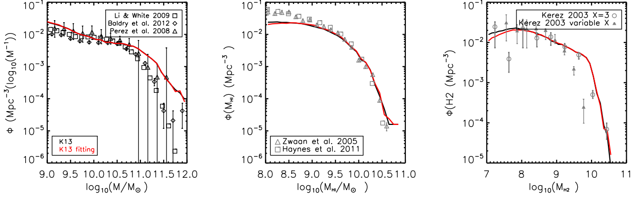
Figure C2. As for Fig. C1 but this time for different assumptions for the density of dark matter and stars ( \rho_{sd} ) within the K13 model. The black lines correspond to our default model described in Section 2.4.3. Red lines correspond to results based on the same physical model but using the lower limit for \rho_{sd} resulting from the fitting function provided by Krumholz (2013).
