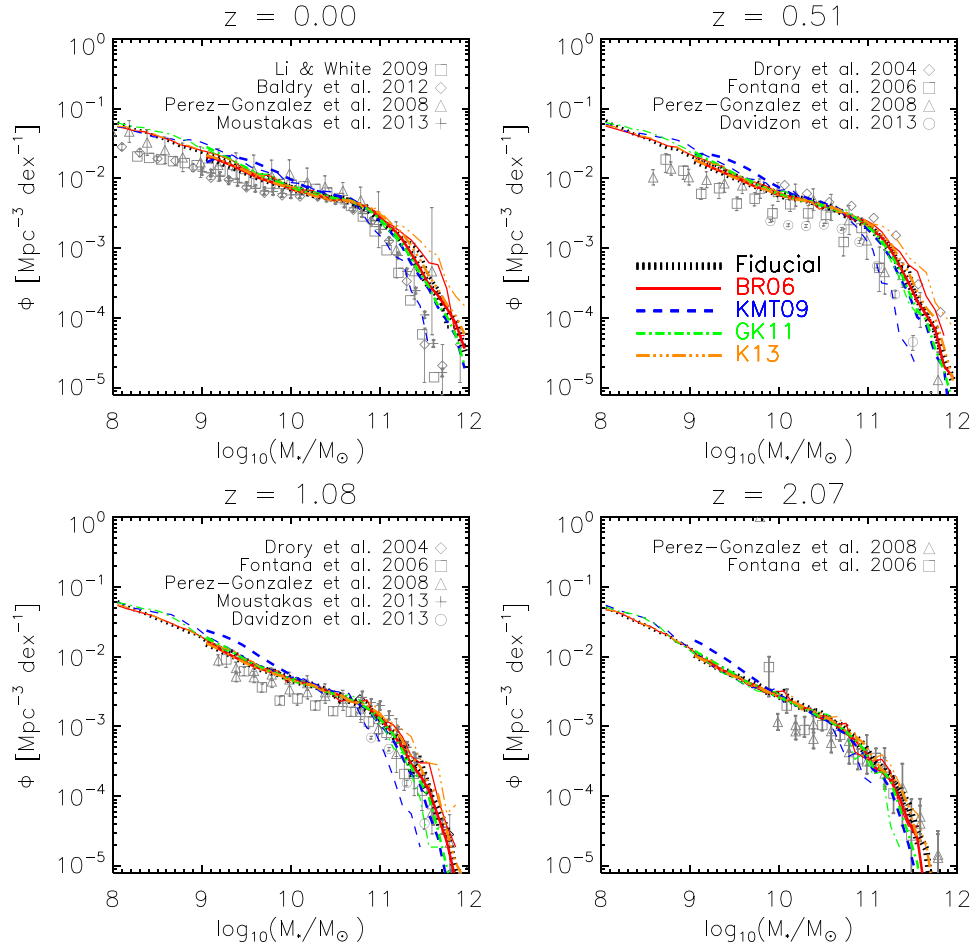
Figure 6. Galaxy stellar mass functions at redshift z = 0 , z \sim 0.5 , z \sim 1 and z \sim 2 . Grey symbols show different observational estimates (Drory et al. 2004; Fontana et al. 2006; Pérez-González et al. 2008; Li & White 2009; Baldry et al. 2012; Davidzon et al. 2013; Moustakas et al. 2013), while lines of different colours and types correspond to different star formation laws, as indicated in the legend. Thicker lines are used for the MS, while thinner lines correspond to the MSII.
