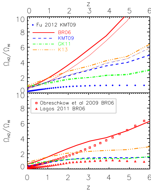
Figure 14. The cosmic molecular ratio \Omega_{\text{H}_2}/\Omega_{\text{H I}} as a function of redshift. Thick curves correspond to our runs based on the MSII, while thin curves correspond to the MS. The red squares, red triangles and blue dots are predictions from Obreschkow & Rawlings (2009b, with BR06), Lagos et al. (2011b, with BR06) and Fu et al. (2012, with KMT09), respectively. The top panel shows results for galaxies above M_* > 10^9 M_\odot . The bottom panel shows results for galaxies with M_* > 10^8 M_\odot .
