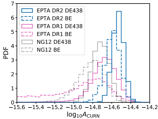
Figure 9. Comparison of the CURN recovered signals with EPTA DR2, DR1 and NG12 (Arzoumanian et al. 2020), using fixed DE438 and BAYESEPHEM with ENTERPRISE and fixed \gamma_{\text{CURN}} = 13/3 .
