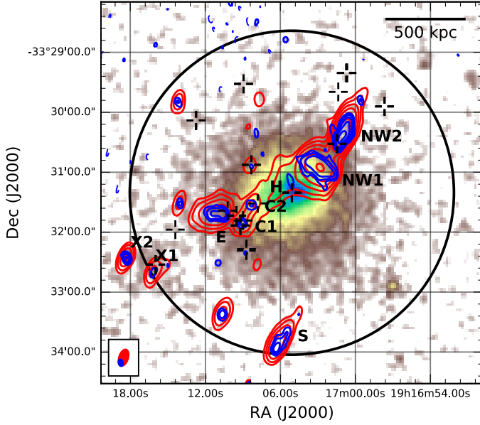
Fig. 2. Same legend as in Fig. 1 except that the red contours are 325 MHz. The 325 MHz beam is 17.5'' \times 9.5'' , and 610 MHz is 7.2'' \times 4.9'' .
