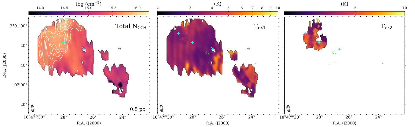
Fig. C.2. Same as Figure C.1, but for clump F1 and F2. White contours in the left panels represent the integrated intensity map of CCH 1 1,1 -0 1,1 line (80-95 km s -1 ), from 2.2 K km s -1 (7 \sigma ) to 6.0 K km s -1 (0.9 times the peak emission of F1) with six uniform intervals.
