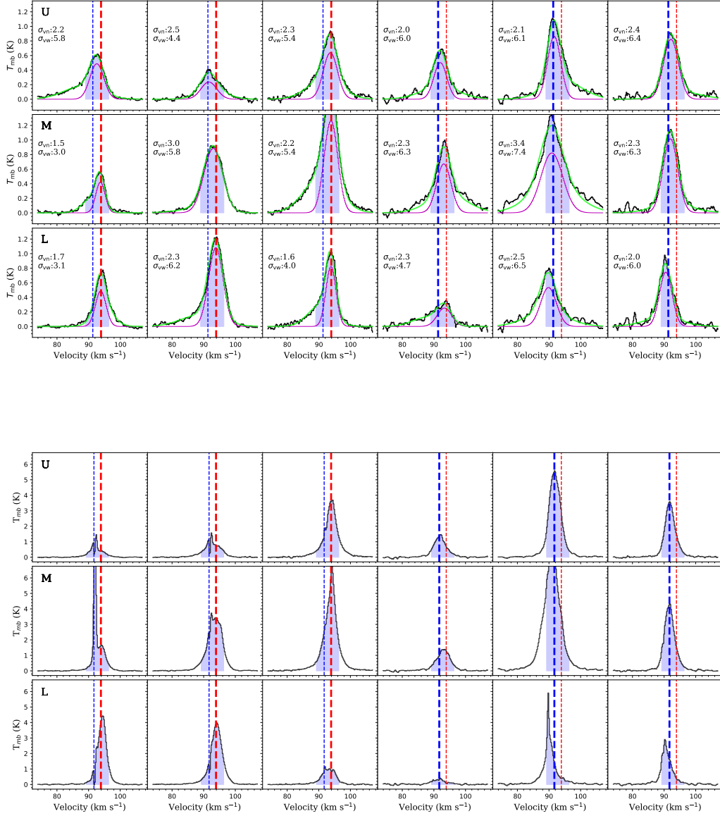
Fig. 10. Average spectra of SiO (2–1) (upper panel) and CH 3 OH 5 1,5 –4 0,4 (lower panel) along the three PV cuts U, M, L as in panel b of Fig. 9. The spectra are arranged from northeast to southwest along the cuts. The blue and red dashed lines indicate the V_{\text{LSR}} of clump MM3 and MM2 (93.9 km s −1 and 91.3 km s −1 ), with the thicker line corresponding to the V_{\text{LSR}} of either clump MM2 or MM3 at this position. The blue shaded regions indicate the line central velocity range from (91.3–2.5) km s −1 to (93.9+2.5) km s −1 , which is excluded from the integration of the intensity maps of panel b in Fig. 9. In the upper plot, the two-component Gaussian fit to the SiO line is shown additionally, as green line. The broad-component subtracted spectrum (narrow-component line profile) is shown as magenta line. The velocity dispersions for the two components are indicated in the figure, in unit of km s −1 .
