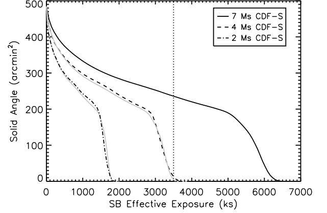
Figure 3. Survey solid angle as a function of minimum soft-band effective exposure for the 7 Ms CDF-S (black solid curve). The vertical dotted line indicates an effective exposure of 3.5 Ms, and 235.9 arcmin 2 (49%) of the 7 Ms CDF-S and 13.0 arcmin 2 (3%) of the 4 Ms CDF-S have > 3.5 Ms effective exposure. For comparison, the dashed and dash-dotted curves display the 4 Ms CDF-S (Xue et al. 2011) and 2 Ms CDF-S (Luo et al. 2008) solid angles, which were derived following the same procedures as in this paper. The 7 Ms curve can be roughly rescaled to 4 Ms and 2 Ms curves with scaling factors of 1.8 and 3.5 in effective exposure (gray solid curves), respectively.
