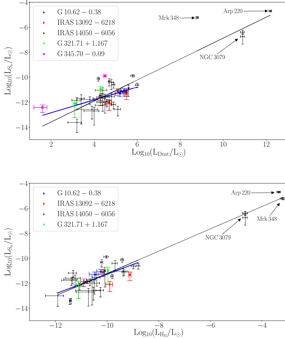
Figure 8. Absorption luminosity of the 6.7 GHz \text{CH}_3\text{OH} line ( L_{S_v} = 4\pi d^2 S_{v,\text{line}} ) as a function of FIR luminosity (upper panel) and 5 GHz radio luminosity (lower panel). Sources identified with different symbols and colours are regions for which the distance ambiguity has not been resolved, and thus, significantly different luminosity values are possible. No interferometric continuum observations of G345.70–0.09 are available, thus, it was not included in the lower panel. All data in the upper panel were fit with an \alpha = 0.84 \pm 0.07 power law (black fit); and the thick slope (blue line) shows the fit ( \alpha = 0.51 \pm 0.14 ) when the extragalactic sources are excluded. The data in the lower panel were also fit with a power law ( \alpha = 0.89 \pm 0.05 ) when all data are included (black fit), and with a power-law \alpha = 0.78 \pm 0.16 when only sources with \log(L_{\text{HI}}/L_\odot) between -12 and -8 are included (thick fit line shown in blue).
