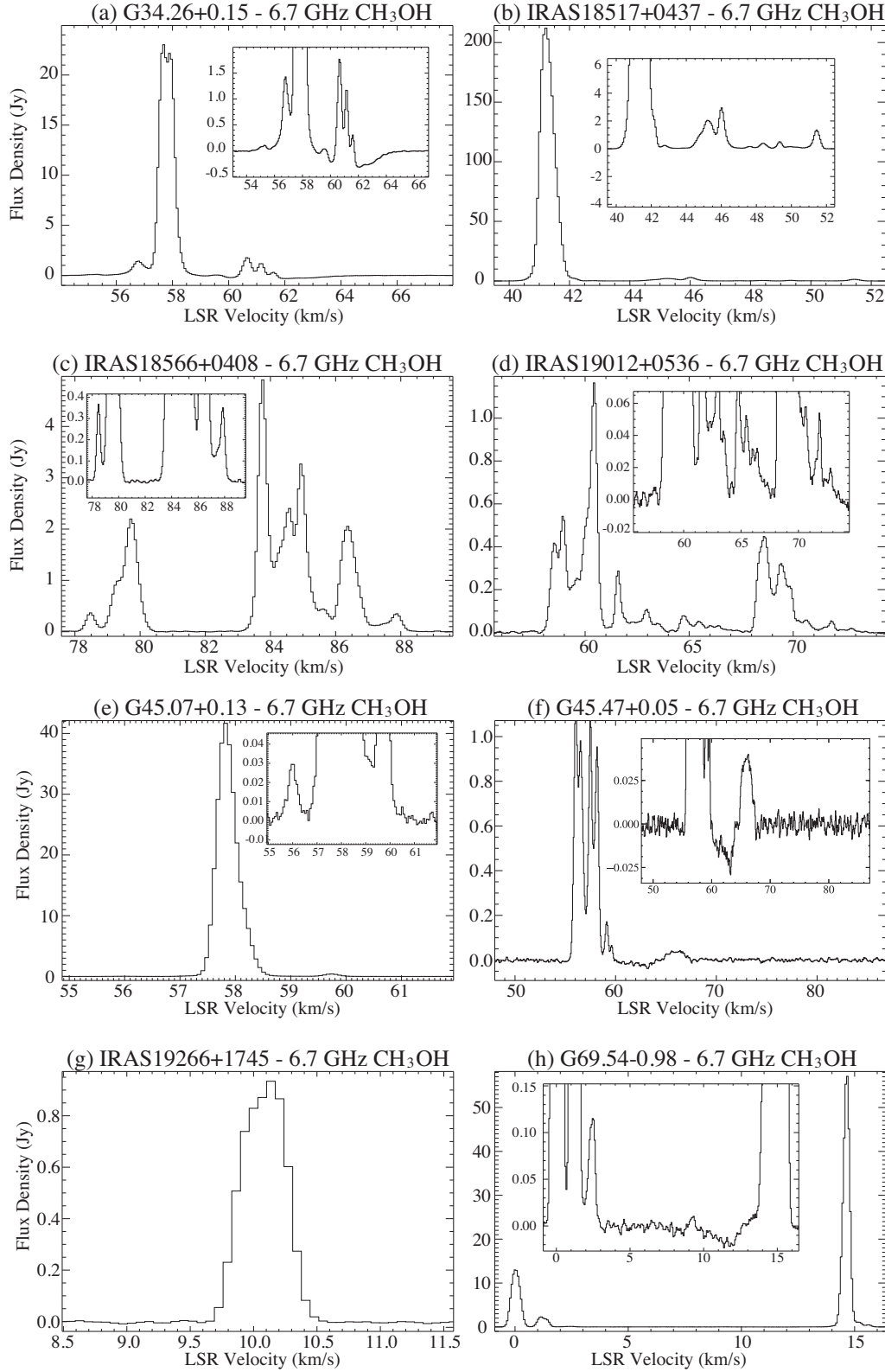
Figure 1. Detection of \text{CH}_3\text{OH} lines toward eight sources (see Table 5; the G45.12+0.13 spectra is shown in Fig. 2). Insets highlight weak masers and/or absorption. The data shown in the figure are available as Supporting Information.
