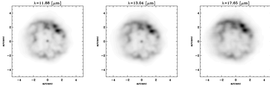
Fig. 1.— VISIR images of IRAS 18576+0341 and its surrounding nebula taken through the filters PAH2 2 , NeII 2 and Q1.
