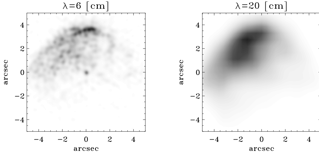
Fig. 6.— Uniform weighted radio maps of IRAS 18576+0341 at 6 and 20 cm, obtained by merging A and C VLA configuration data.
