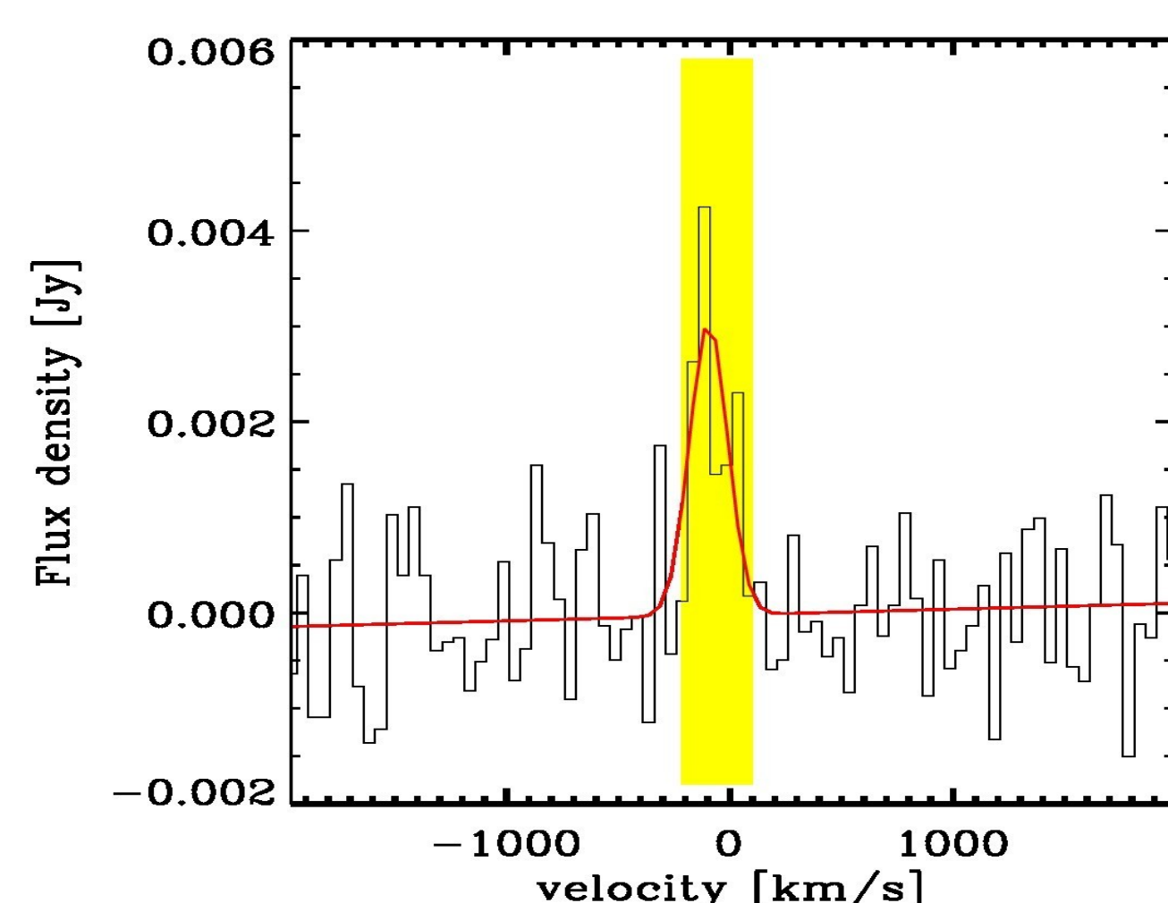
Fig. 5: CO(2-1) spectra of one of our sample and the corresponding moment 0 map in channels shaded by yellow
