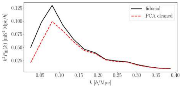
Fig. 36 Measured H I power spectra demonstrating the H I signal loss effect after foreground cleaning with PCA ( N_{\text{FG}} = 3 ). This figure was produced using the publicly available code IntensityTools (Cunnington et al. 2019; Blake 2019; Soares et al. 2021) and MeerKAT-like simulated data products at 0.2 < z < 0.58
