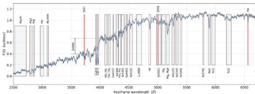
Fig. 3 Stacked spectrum of \sim 100,000 massive and passive CC selected from SDSS DR12. It is possible to see clearly how it is characterized by a red continuum, several absorption lines (identified by the black boxes), and by the absence of significant emission lines (whose position is highlighted by the red boxes)
