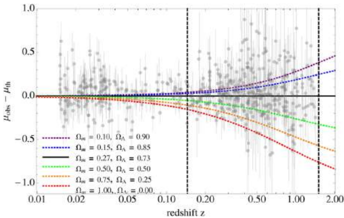
Fig. 11 Residual distance modulus for different values of the density cosmological parameters up to z = 2.0 . We consider the best fit to be the standard \Lambda CDM model, where \Omega_m = 0.27 , \Omega_\Lambda = 0.73 , and \ddot{a} = 71 \text{ km s}^{-1} \text{ Mpc}^{-1} (black line). Union2 SNe Ia data residuals are shown in grey. The large spread (more than 1 mag) shown by \mu at z = 1.5 and at z = 0.145 (the two vertical dashed lines) where the scatter is almost 0.2 mag is clearly evident. Image reproduced with permission from Izzo et al. (2015), copyright by ESO
