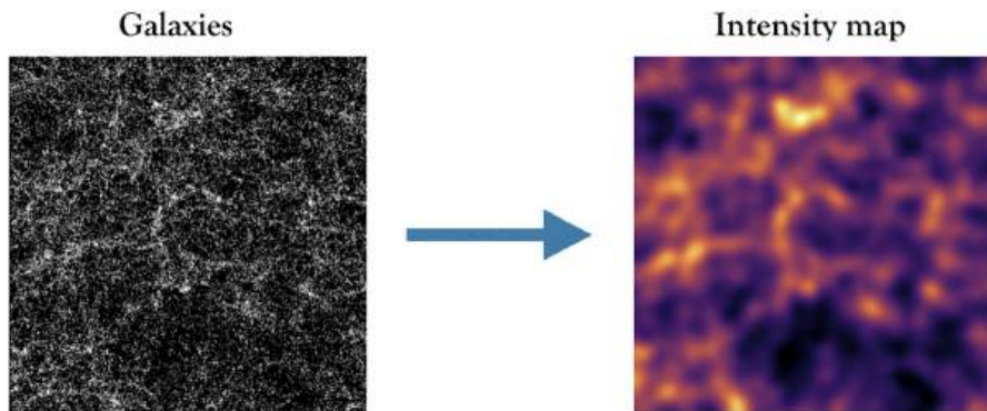
Fig. 32 From individual galaxies (left) to H I intensity maps (right). Using the intensity mapping technique we can map the entire H I flux from many galaxies together in large 3D pixels, and produce low angular resolution H I brightness temperature maps that retain the large-scale statistical information. This figure was produced using the MultiDark simulations (Klypin et al. 2016; Knebe et al. 2018) and the methods in Cunningham et al. (2020b)
