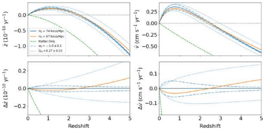
Fig. 46 Secular redshift drift (left) and apparent acceleration (right) versus redshift. All loci assume H_0=74 \text{km s}^{-1} \text{Mpc}^{-1} , \Omega_m=0.27 , \Omega_\Lambda=0.73 , and w_0 = -1 unless otherwise indicated. The top row shows the full signal, and the bottom row shows the difference between several models and the fiducial cosmology
