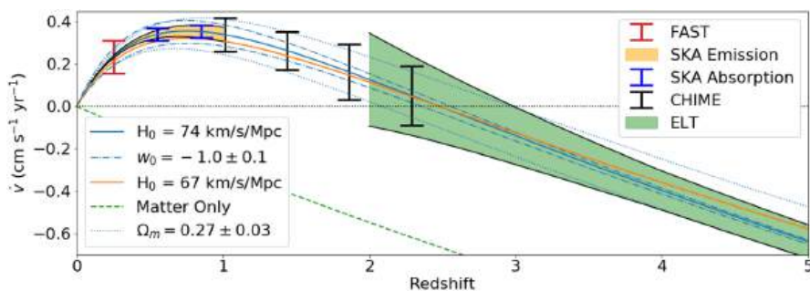
Fig. 47 Forecast acceleration measurements versus redshift for the SKA using H \text{i} 21-cm emission from galaxies (Kloekner et al. 2015), CHIME using H \text{i} 21-cm absorption (Yu et al. 2014), H \text{i} 21-cm absorption using FAST and the SKA estimated from projected detections (see text), and an ELT program that monitors the Ly \alpha forest (Liske et al. 2008). The cosmological tracks follow Fig. 46. The shaded loci and error bars indicate 1\sigma uncertainties
