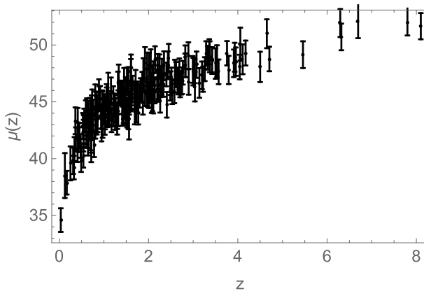
Fig. 15 GRB Hubble diagram build up by calibrating the E_{p,i} – E_{iso} correlation for the updated sample of 208 GRBs used for this review
