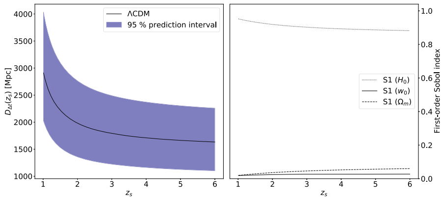
Fig. 24 Similar to Fig. 23, but showing the sensitivity of the time-delay distance, D_{At}(z_s) , to the values of the cosmological parameters H_0 , \Omega_m , and w_0
