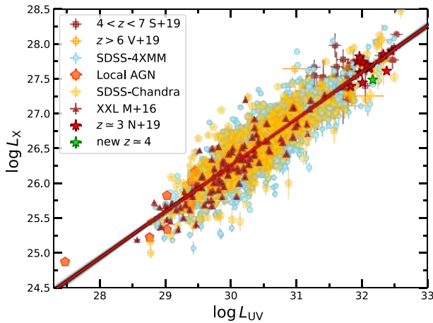
Fig. 8 The L_X - L_{UV} relation for the \simeq 2400 quasars published by Lusso et al. (2020). Symbol keys are the same as in Fig. 7. The red line represents the linear regression fit of the data obtained through the hierarchical Bayesian model linmix (Kelly 2007). The light black lines represent some random realisations of the L_X - L_{UV} relation. The resulting slope and intercept of the best-fit regression line are \gamma = 0.667 \pm 0.007 and \beta = 6.25 \pm 0.23 . The observed dispersion along the L_X - L_{UV} relation is 0.24 dex. Luminosity values are computed by assuming a flat \Lambda CDM model with \Omega_M = 0.3
