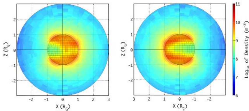
Figure 3: The O_2 exosphere of Ganymede generated due to the radiolytic decomposition of ice being impacted by Jupiter's magnetospheric ions to ( S^+ , O^+ and H^+ ). Top panel shows the exospheric density distribution at the XZ plane ( X is along the ambient flow direction and Ganymede's orbital motion and Z is along the Jupiter's spin axis (in units of Ganymede's radii)); middle panel refers to the XY plane ( Y points towards Jupiter (in unit of Ganymede's radii)); bottom panel shows the trailing hemisphere exosphere in the YZ plane.
