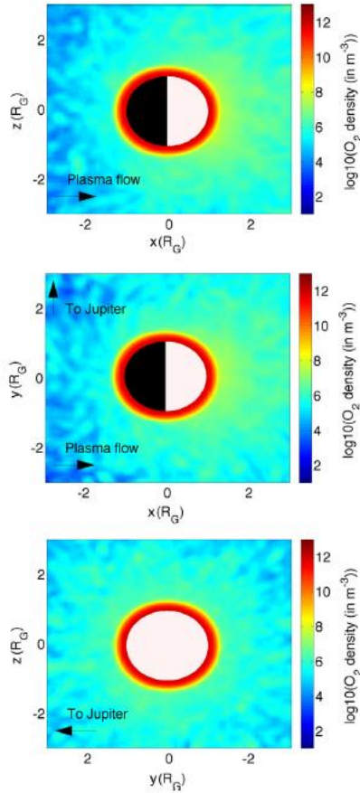
Figure 3: The O_2 exosphere of Ganymede generated due to the radiolytic decomposition of ice being impacted by Jupiter's magnetospheric ions to ( S^+ , O^+ and H^+ ). Top panel shows the exospheric density distribution at the XZ plane ( X is along the ambient flow direction and Ganymede's orbital motion and Z is along the Jupiter's spin axis (in units of Ganymede's radii)); middle panel refers to the XY plane ( Y points towards Jupiter (in unit of Ganymede's radii)); bottom panel shows the trailing hemisphere exosphere in the YZ plane.
