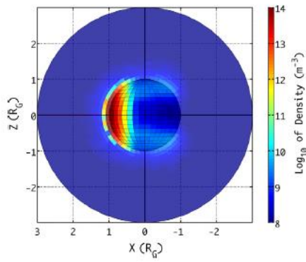
Figure 5. In this case, the position of Ganymede along its orbit is important; we have frozen the simulation at the time when the Sun is in the +x direction (the illuminated side corresponds to the leading one). The exosphere density is up to \sim 2.5 \cdot 10^{14} \text{ m}^{-3} in the sub-solar point.
