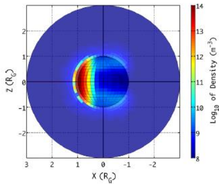
Figure 5: XZ projection of the \text{H}_2\text{O} exosphere density due to sublimation and sputtering over the surface of Ganymede. X is along the ambient flow direction (and Ganymede's orbital motion), Z is along the Jupiter's spin axis, and Y points toward Jupiter (in units of Ganymede's radii). The Jupiter-facing hemisphere is shown (the illuminated leading hemisphere is on the left). It is clear that the sputtered exosphere is much less intense close to subsolar point, while it is the major generation process in the rest of the moon.
