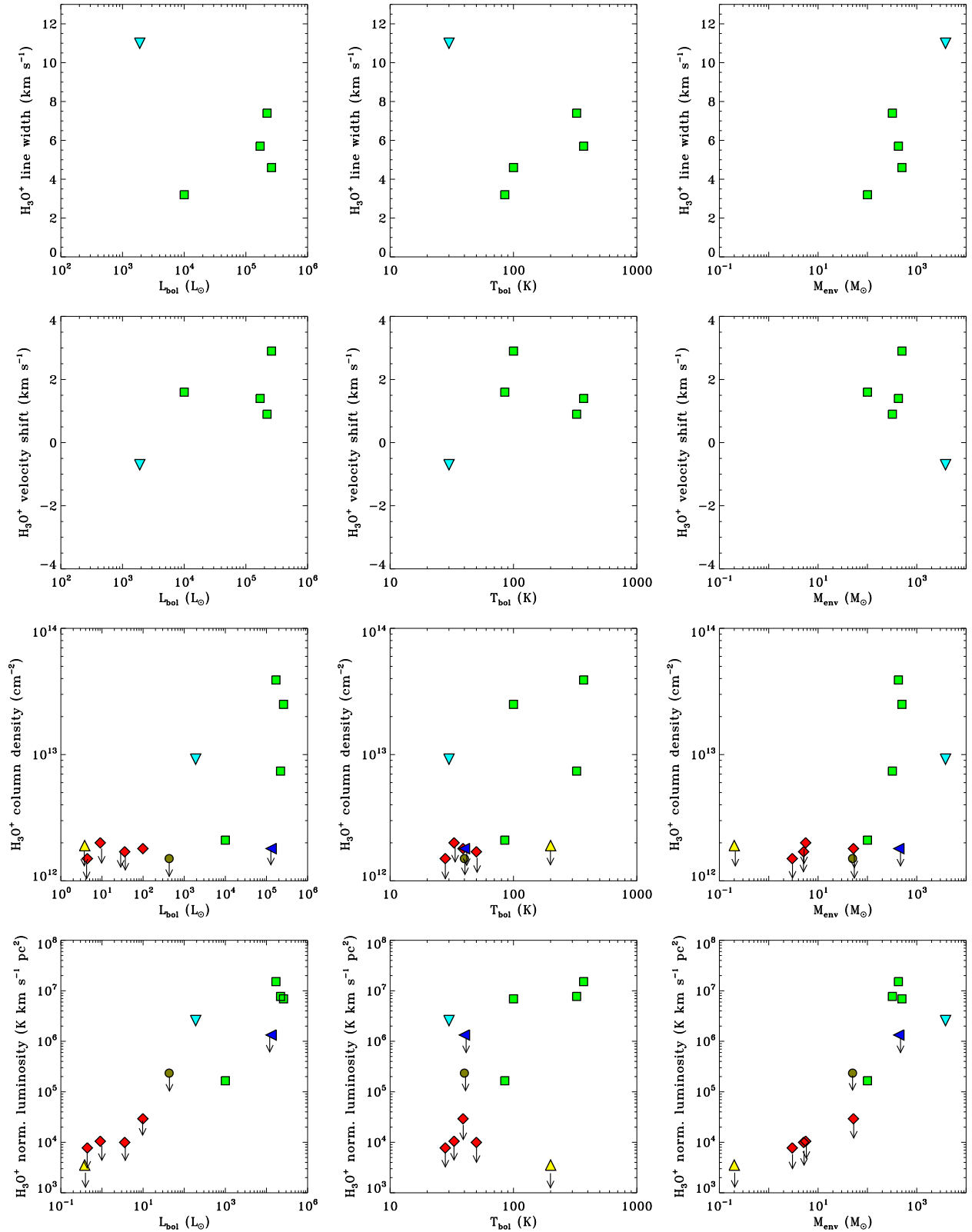
Fig. C.6. Observed \text{H}_3\text{O}^+ (1031 GHz) line characteristics (Table B.1) vs. object parameters given in Table 1. The line is in emission. The bottom row shows the line luminosity multiplied with distance squared (normalized to 1 pc) to correct in case of point-source emission. The symbols mark different types of objects: red diamonds for Class 0, yellow triangle up for Class I (L 1489), brown circle for intermediate mass, light blue triangle down for high-mass mid-IR quiet (NGC 6334 I(N)), green square for high-mass mid-IR bright and hot molecular core, and dark blue triangle left for high-mass ultra-compact HII (NGC 7538 IRS1).
