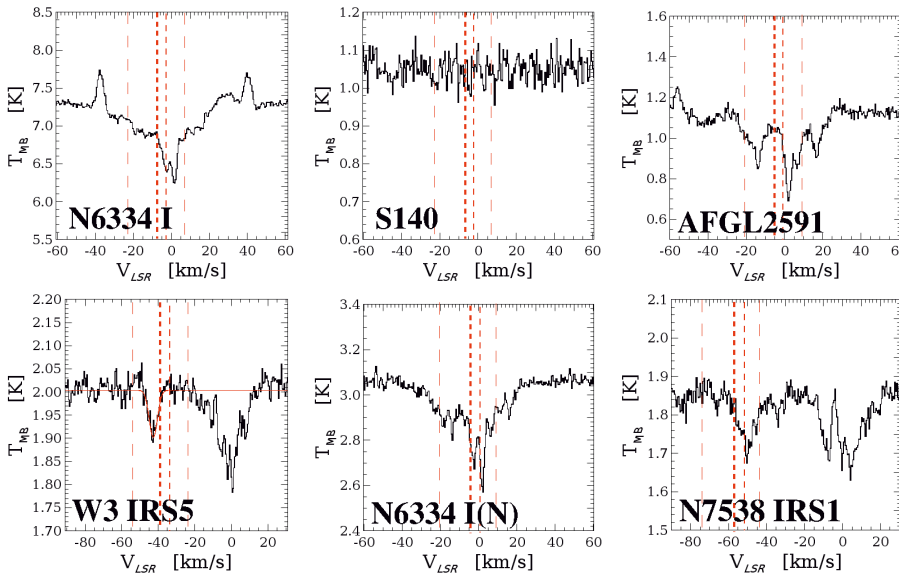
Fig. A.4. Ortho- \text{H}_2\text{O}^+ ( N_{KaKaJ} = 1_{11\frac{3}{2}} - 0_{00\frac{1}{2}} ) lines at 1115 GHz observed toward the high-mass objects. The position of the strongest lines shifted by the systemic velocity of the YSO is indicated with vertical red dashed lines. Their thickness indicates the theoretical intensities. Only the blue-shifted line of W3 IRS5 is fitted by a Gaussian (red, see text). Its parameters are given in Table B.1.
