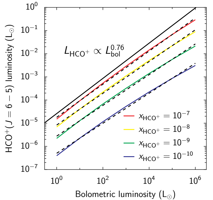
Fig. D.3. L_{\text{bol}} vs. L_{\text{HCO}^+}(J = 6-5) relation (full curves). The color indicates the 4 different HCO + abundances used. The model results are compared to the observed L_{\text{HCO}^+} \propto L_{\text{bol}}^{0.76 \pm 0.08} power-law, indicated by a black solid line at the top (in arbitrary units) and power-law fits to the model relation (black dashed lines).
