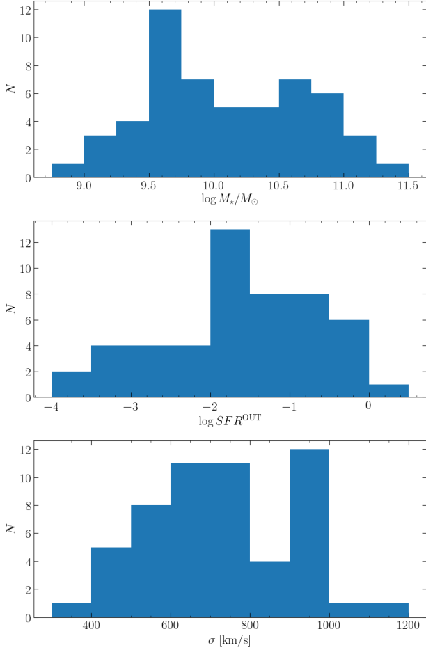
Figure 2. Distribution of the stellar mass (upper panel), SFR in the tails (central panel) and velocity dispersion of the host cluster (lower panel) for the sample galaxies.
