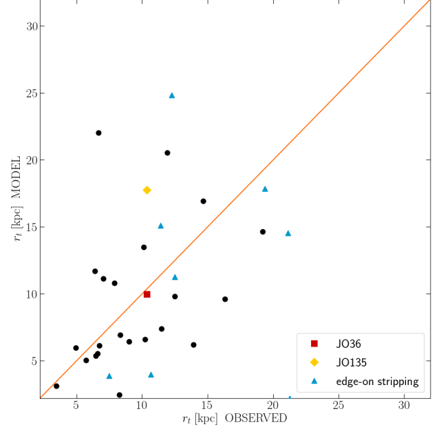
Figure 7. The truncation radius r_t computed using the model described in Sect. 5 compared with the value estimated from our observations. The diagonal line is the 1:1 relation. Symbols are as in Fig.9
