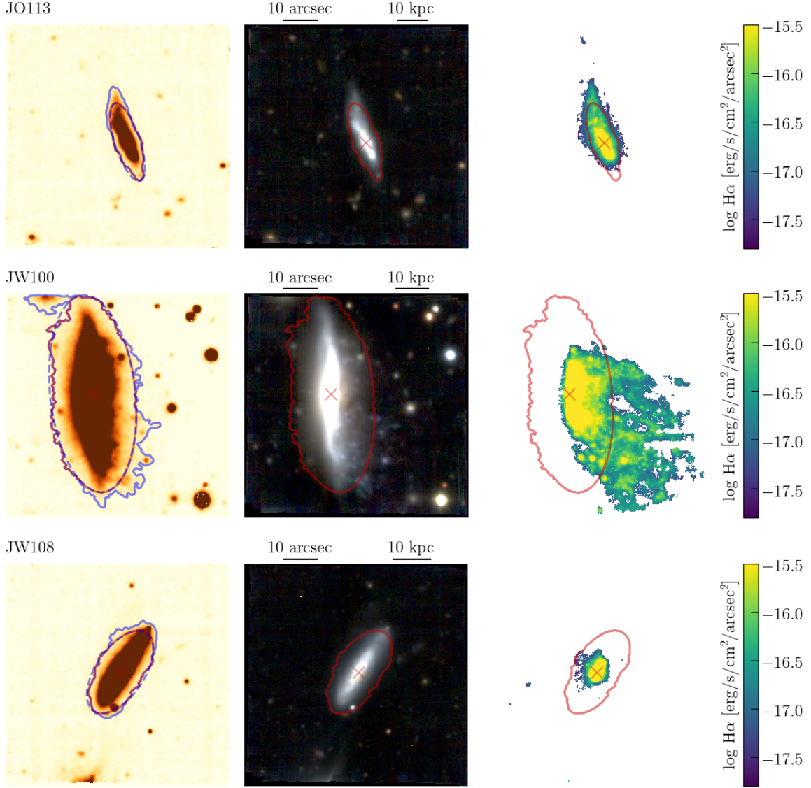
Figure 1. From left to right: (i) the continuum emission in the H\alpha region; (ii) an RGB image obtained from g -, r -, and i -band images derived from the MUSE datacube; (iii) the H\alpha emission of three galaxies at different stripping stages: JO113 (moderate stripping), JW100 (jellyfish galaxy), and JW108 (truncated disc or post stripping). The blue line is the isophote corresponding to a continuum surface brightness 1\sigma above the background level; the dashed line is the ellipse that better describes the isophote on the undisturbed side of the galaxy and the red line is the resulting line that we used to define the galaxy main body. The same figure for all galaxies is available at http://web.oapd.inaf.it/gasp/inandout .
