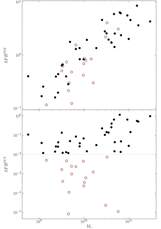
Figure 3. Total SFR (upper panel) and SFR in the tails (lower panel) as a function of the galaxy stellar mass. Red circles shows galaxies with SFR in the tail smaller than 10^{-2} M_\odot \text{ yr}^{-1} .
