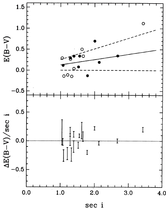
FIG. 3. Upper panel: E(B-V) as a function of the secant of the inclination of the parent galaxy disk. Filled and open circles are points with E(B-V) uncertainties lower and higher than 0.1, respectively. The solid line represents the best fit given in Eq. (5) and corresponds to a selective extinction half-width of 0.13 \pm 0.04 mag. Lines corresponding to slopes 0 and twice the average are also shown. Lower panel: Residuals relative to the average as a function of \sec i . The error bars denote the 1\sigma uncertainties of the individual points. The dispersion corresponds to \text{rms} = 0.15 \pm 0.01 .
