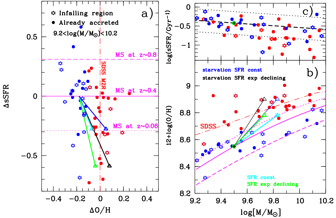
Fig. 9. Panel a): offsets \Delta \text{O/H} to the local MZR vs. \Delta \text{sSFR} to the MS at z \sim 0.4 for cluster galaxies with masses 9.2 < \log(M/M_\odot) < 10.2 ( M_{\text{med}} ). Filled circles (stars) indicate accreted (infalling) galaxies based on their position in the phase-space diagram (Fig. 7). Galaxies with O/Hs consistent with the local MZR are shown in red, other objects in blue. The MS mean values at z \sim 0.8 , z \sim 0.4 , and z \sim 0.06 , based on the equation of the evolution of the sSFR from Peng et al. (2010a), are indicated by dashed, solid, and dotted magenta lines. The dash-dotted red line indicates the median local MZR of our matched SDSS sample (see also Fig. 5). Four tracks of a model galaxy start with 1.2 \text{ M}_\odot/\text{yr} and \log(M/M_\odot) = 9.5 . The model galaxy continues forming stars for 3 Gyr with a constant SFR (cyan track) or exponentially declining SFR with a \tau = 3 Gyr (green track), and the corresponding tracks are shown for a strangulation scenario with constant SFR (blue track) and exponentially declining SFR (black track). Panel b): MZR for M_{\text{med}} cluster galaxies with data symbols and paths of model galaxies color-coded as in panel a). The magenta lines show the Li13 expectations of the Z(M, \text{SFR}) for galaxies on the MS at different redshifts, with dashed, solid, and dotted lines corresponding to different z like the magenta lines in the panel a). Panel c): the mass-sSFR relation for cluster galaxies color-coded in red for O/Hs consistent with the local MZR. Dashed and dotted lines show the median and dispersion of the mass-sSFR relation according to Peng et al. (2010a). The green filled circles with a black cross in panels b) and c) indicate the starting point of the toy models described in Sect. 5.2: \log(M_{\text{start}}/M_\odot) = 9.5 , \text{SFR}_{\text{start}} = 1.2 \text{ M}_\odot/\text{yr} , and Z_{\text{start}} = 8.55 . For the sake of visibility we do not plot error bars in Fig. 9; however, the error bars were already shown in the respective mass-sSFR (Fig. 3) and MZR plot (Fig. 5) for galaxies of all stellar masses.
