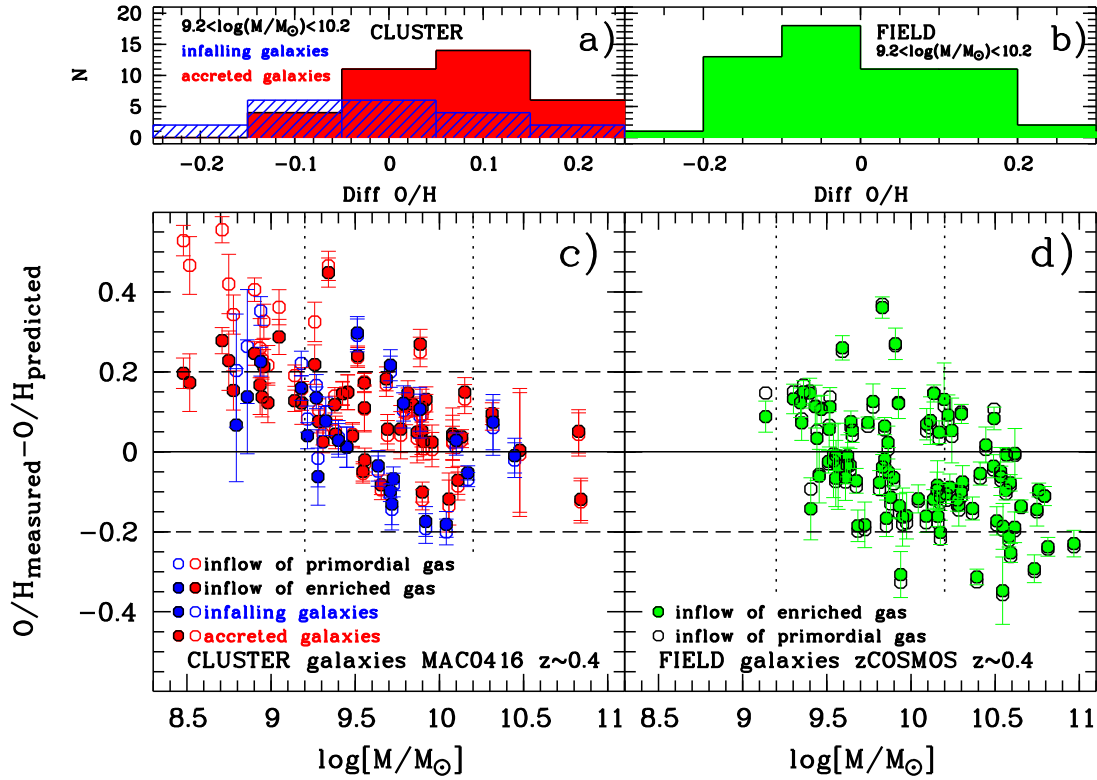
Fig. 8. Difference between the measured O/Hs of z \sim 0.4 Zgals cluster galaxies (panel c) and zCOSMOS field objects (panel d) and the expected O/Hs from the formulations of Li13 for different infall metallicities Z_0 relative to the yield y , Z_0/y = 0.1 (enriched inflow, filled circles) and Z_0/y = 0 (pristine inflow, open circles). In addition, in panel c) the position of cluster galaxies in the phase-space diagram (see Fig. 7) is indicated in red (blue) for accreted (infalling) galaxies. The upper histograms (panels a) and b)) for M_{\text{med}} objects show that in general the infalling cluster members (blue histogram) and field galaxies (panel b)) have lower metallicities, in quite good agreement with the FMR, unlike accreted galaxies (red histogram), which in general have higher metallicities than predicted by the FMR.
