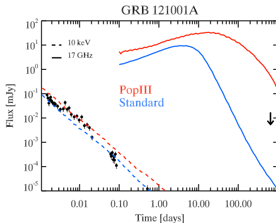
Figure 3. Example of how the simulated X-ray light curves (dashed lines) can reproduce equally well the X-ray observed data (black dots). The simulation is then run at 17 GHz (solid lines), keeping all parameters fixed, and the difference in behaviour becomes evident. The left-hand (right-hand) panel shows GRB 121001A (GRB 110210A), respectively. The ATCA upper limits obtained with our pilot program are shown with a vertical arrow. The two scenarios investigated are plotted with different colours.
