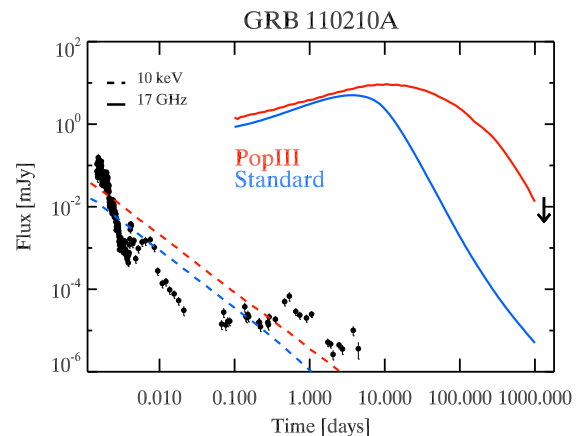
Figure 3. Example of how the simulated X-ray light curves (dashed lines) can reproduce equally well the X-ray observed data (black dots). The simulation is then run at 17 GHz (solid lines), keeping all parameters fixed, and the difference in behaviour becomes evident. The left-hand (right-hand) panel shows GRB 121001A (GRB 110210A), respectively. The ATCA upper limits obtained with our pilot program are shown with a vertical arrow. The two scenarios investigated are plotted with different colours.
