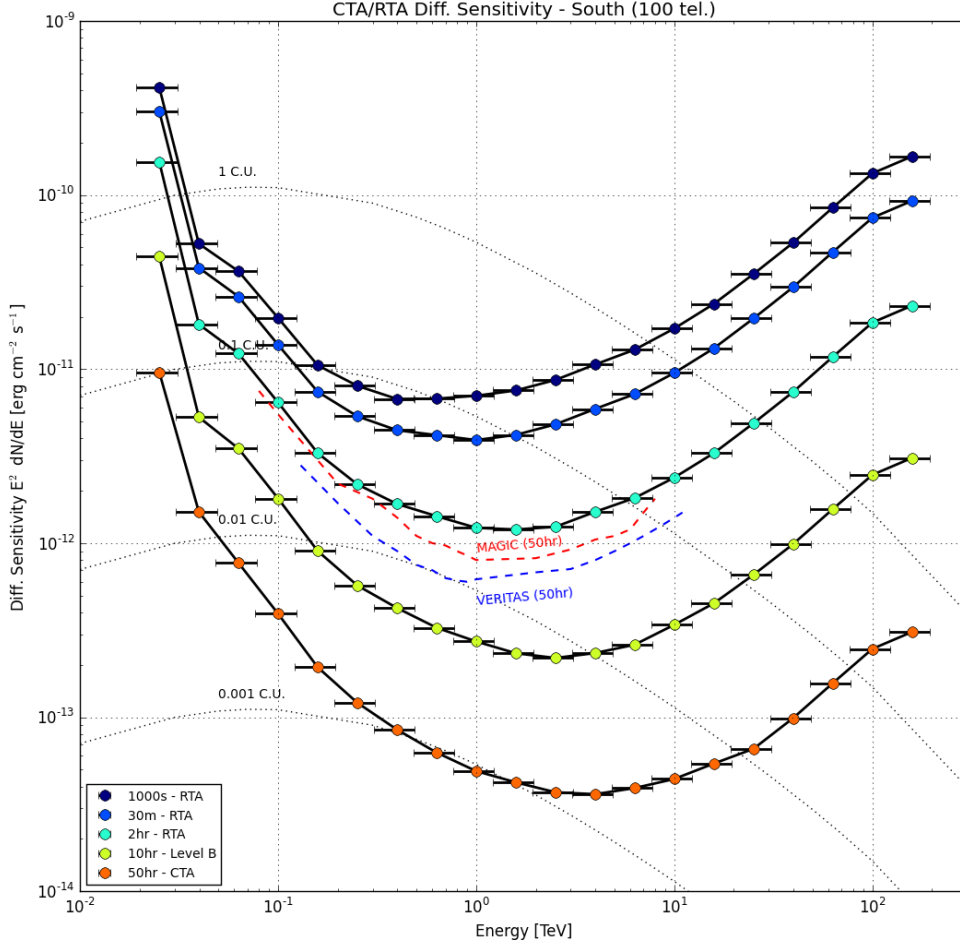
Figure 1: Differential sensitivity, in \text{erg cm}^{-2} \text{ s}^{-1} , of the Real-Time and Level B analysis pipelines computed for t_{\text{exp}} = 1000\text{s} , 30m, and 2hr (RTA) and 10hr (Level B). The expected CTA sensitivity is also shown for t_{\text{exp}} = 50\text{hr} as reference. The dotted lines show the Crab flux in 0.001, 0.01, 0.1, 1, and 10 C.U., while the dashed lines show the MAGIC and VERITAS sensitivity for a t_{\text{exp}} = 50\text{hr} exposure.
