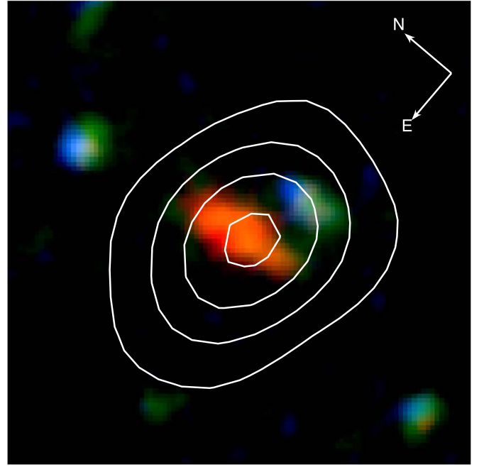
Figure 1. A 3''.0 \times 3''.0 composite image centered at the position of CEERS-DSFG-1; the JWST/NIRCam F115W observations are in blue, F277W in green, and F444W in red (the data have been smoothed to roughly match the F444W resolution for better visualization). The 1.1 mm NOEMA signal-to-noise ratio levels starting at 2.5\sigma to 10\sigma (in steps of 2.5\sigma ) are represented by the white contours, clearly indicating that the dust thermal emission detected at submillimeter/millimeter wavelengths corresponds to the position of CEERS-DSFG-1.
