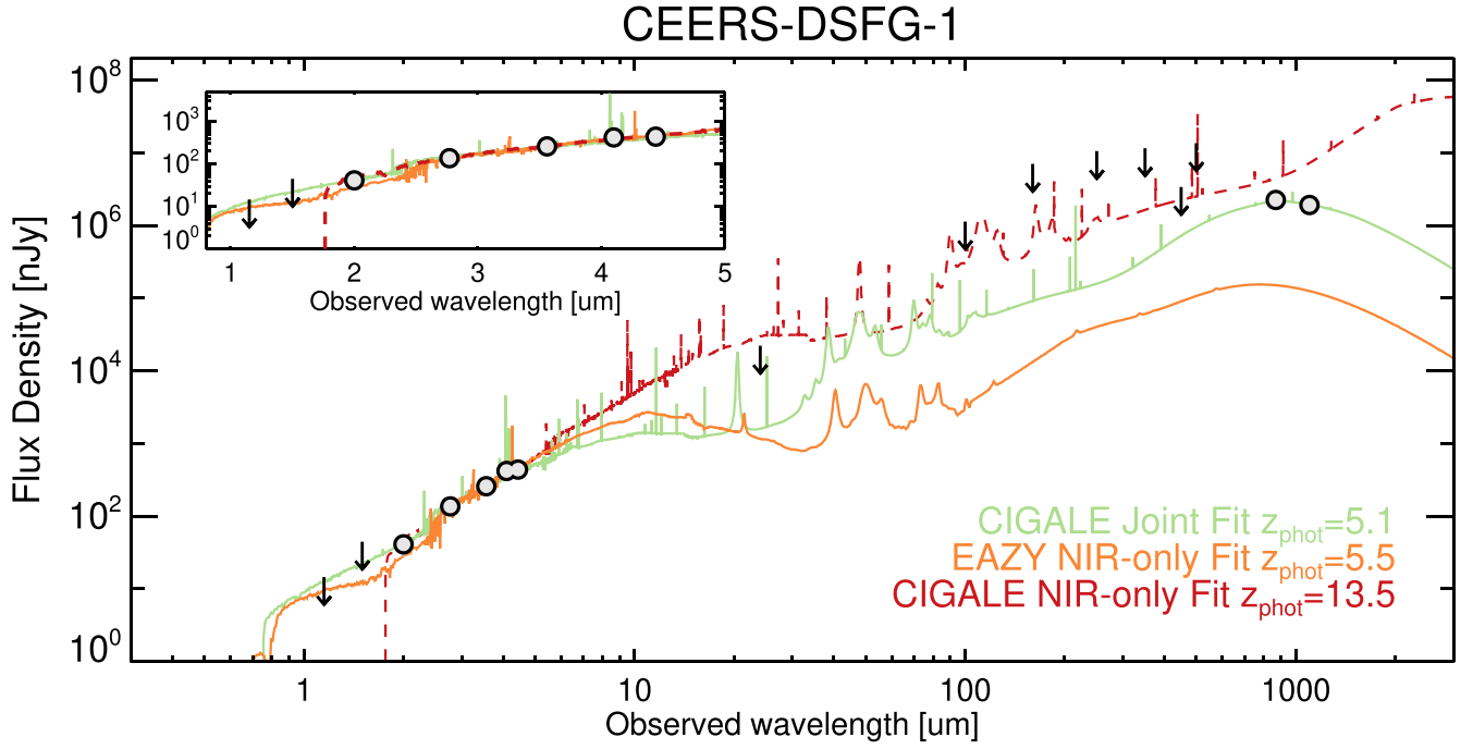
Figure 4. The full near-infrared through millimeter spectral energy distribution of CEERS-DSFG-1 overplotted with several of the best-fit SEDs described in Section 3 along with the current photometric constraints. The detections used in the fits are represented by the solid circles, while 2\sigma upper limits are illustrated by the downward arrows (note that error bars are smaller than the symbols). We show the EAZY fit to near-IR data only at z = 5.5 in orange, CIGALE to near-IR data only at z = 13.5 in red, and the fiducial CIGALE joint fit at z = 5.1 in light green. While the three SEDs satisfactorily reproduce the JWST photometry (see zoom-in inset plot), only the joint fit at z = 5.1 reproduces the (sub)millimeter fluxes.
