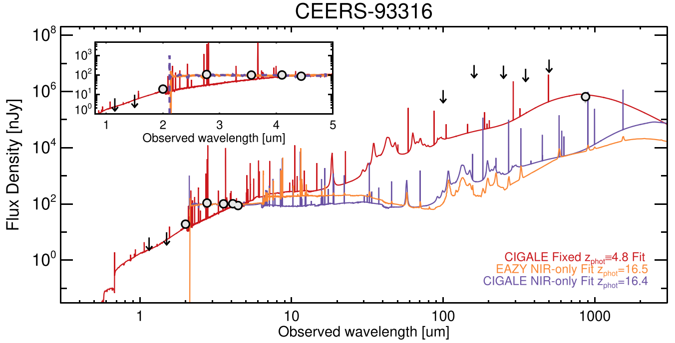
Figure 7. Best-fit spectral energy distributions for CEERS-93316. The orange and purple lines represent the z \sim 16.4 EAZY and CIGALE fits to the near-IR data only, which predict a 850\text{ }\mu\text{m} flux density significantly lower than the value implied by the tentative SCUBA-2 detection. On the other hand, the best-fit SED at z = 4.8 from CIGALE (red line) can reproduce both the near-IR and the submillimeter data. In this case, the blue NIRCcam colors are produced by the strong emission lines, as clearly seen in the inset plot.
