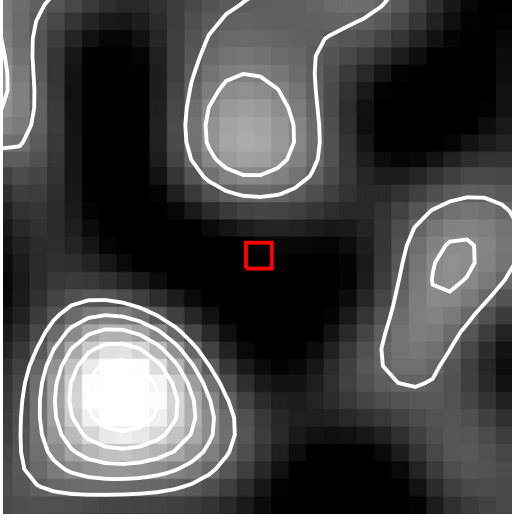
Figure 8. SCUBA-2 850\text{ }\mu\text{m} signal-to-noise ratio map ( 60''0 \times 60''0 ) centered at the position of Maisie's galaxy (red square; Finkelstein et al. 2022a). At the depth of the observations ( \sigma_{850\text{ }\mu\text{m}} = 0.46\text{ mJy beam}^{-1} ), no significant dust emission is detected (the flux density at the position of the source is measured to be -0.4 \pm 0.25\text{ mJy beam}^{-1} ). There is also no statistical significant emission in the available Spitzer (8 and 24\text{ }\mu\text{m} ), Herschel (100– 500\text{ }\mu\text{m} ), or SCUBA-2 ( 450\text{ }\mu\text{m} ) maps.
