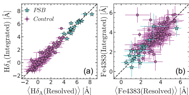
Figure 3. We find very good agreement between the median of the spatial measurements and the measurement on the integrated slit profile, for both H\delta_A and Fe4383 (panels a and b, respectively). The cyan stars are PSB galaxies, and the magenta circles are the control sample of quiescent galaxies (the errorbars have been rescaled). The best-fitting relations have slopes of 0.96 \pm 0.03 (for H\delta_A ) and 1.03 \pm 0.08 (for Fe4383), consistent with unity. The observed scatter about the best-fitting relations is \Delta = 0.26 and \Delta = 0.52 , respectively, consistent with the measurement uncertainties (after rejecting 3\sigma outliers, the reduced \chi^2 value is 1.01 in both cases).
