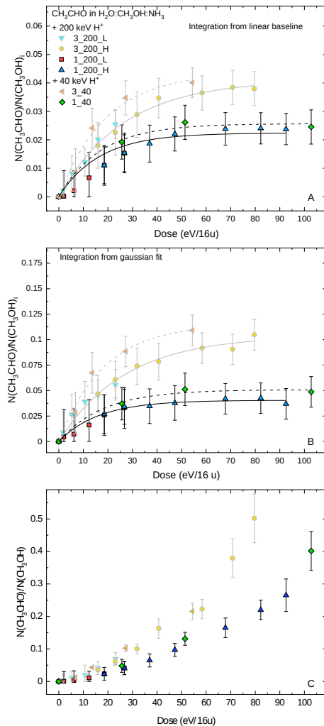
Fig. 6. CH 3 CHO column density with respect to the initial methanol abundance ((CH 3 OH) i , panels A and B ) or during irradiation (CH 3 OH, panel C ). Estimates are based on the analysis of the 1350 cm -1 band for CH 3 CHO and on the 1025 cm -1 band for CH 3 OH. Panel A : estimates obtained after the subtraction of a linear baseline between 1360 and 1330 cm -1 and integration of the 1350 cm -1 band intensity. Panel B : estimates obtained from the integration of Gaussian curves centred at about 1350 cm -1 obtained after a multi-Gaussian fit performed in the range 1500–1300 cm -1 . Panel C : CH 3 CHO with respect to the amount of CH 3 OH during irradiation. The ratio is calculated using the abundances of CH 3 CHO obtained with the method of the integration from linear baseline.
