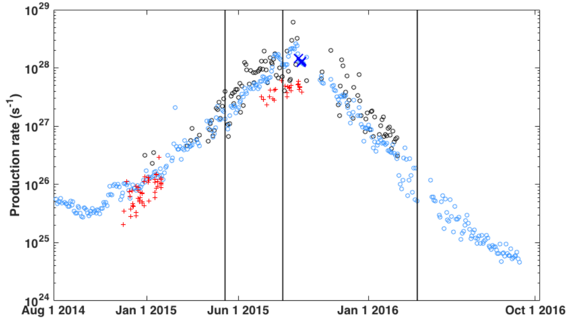
Figure 7. Comparison of Rosetta water production rates in comet 67P/Churyumov-Gerasimenko. The red +’s are the same water production rates in Figure 6 obtained by interpreting the VIRTIS-H measurements of Bockelée-Morvan et al. (2015 and 2016) with the ROSINA DFMS determined water potential surface distribution model. The blue circles are also the same two-day average values from the ROSINA DFMS measurements. The black circles are two-day averages determined from the column densities from the MIRO observations of Marshall et al. (2017) also using the coma distributions from our ROSINA DFMS determined water surface distribution. The blue X’s are determined from the H Ly \alpha observations by Shinnaka et al. (2017), the sizes of which are indicative of the given uncertainties. The vertical lines left to right represent the first equinox, perihelion, and second equinox, respectively.
