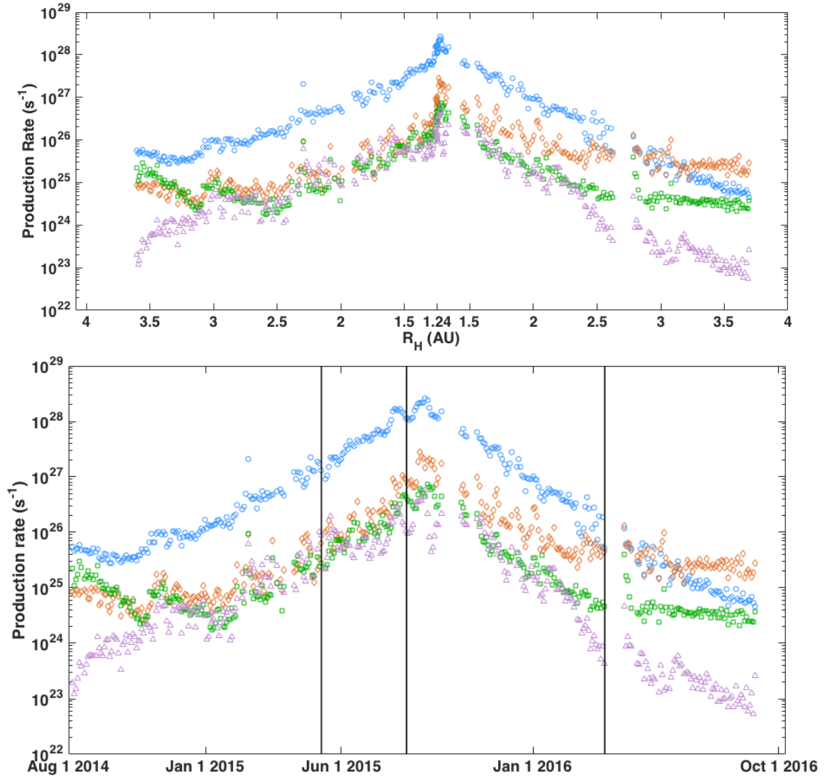
Figure 5. Production rates of \text{H}_2\text{O} (blue), \text{CO}_2 (orange), \text{CO} (green), and \text{O}_2 (purple) throughout the mission as a function of heliocentric distance, R_H in AU (top), and as a function of time (bottom). The vertical lines represent the first equinox, perihelion, and second equinox, respectively.
