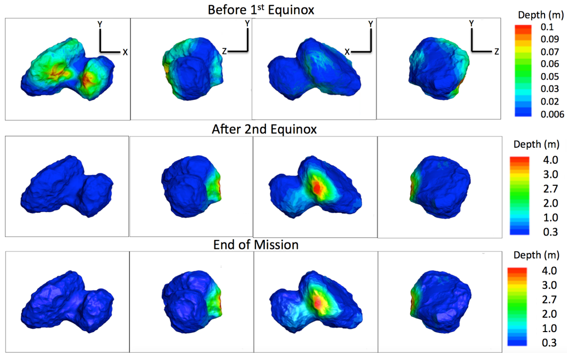
Figure 9. Cumulative Erosion Depths at the end of each of three mission phases: 1st equinox, after 2nd equinox and end of mission. Note that by necessity the color contour look-up table is different for the first phase. A dust/gas (or refractory/ice) loss ratio of 1:1.5 is assumed for a nucleus of density 533 \text{ kg m}^{-3} . Results can be scaled for other ratios.
