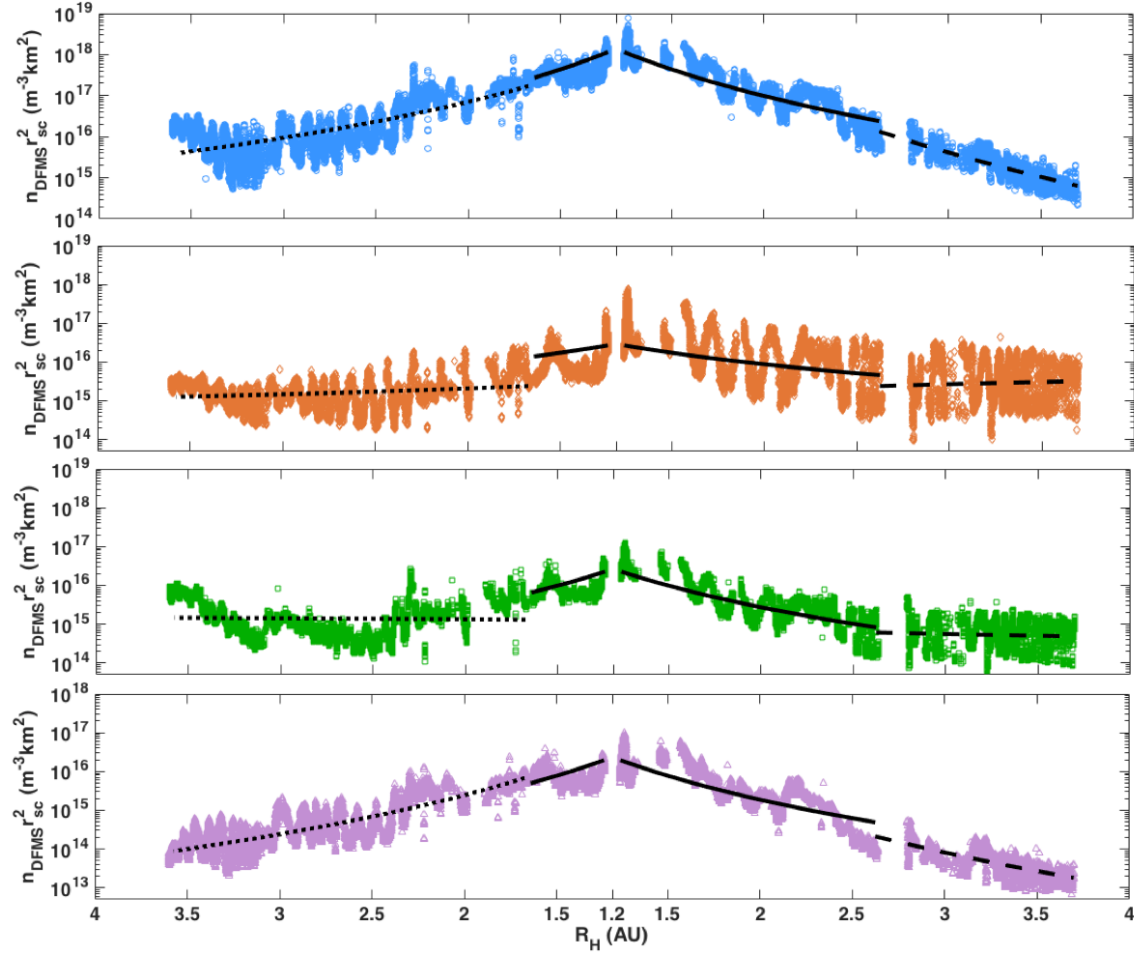
Figure 1. Heliocentric distance dependence of DFMS densities normalized by the inverse square of the spacecraft-comet distance. From the top down the plots are for the \text{H}_2\text{O} (blue), \text{CO}_2 (orange), \text{CO} (green) and \text{O}_2 (purple). The lines in each give the power-law fits for the three separate time periods as given in Table 1, dotted for phase 1, solid for phase 2 and dashed for phase 3.
