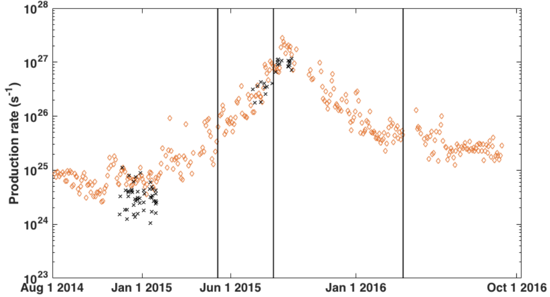
Figure 6. Comparison of production rates of CO 2 determined from the ROSINA DFMS data (orange circles) with those from VIRTIS-H (black x's) from the observations of Bockelée-Morvan et al. (2015 and 2016) using the spatial distributions from the DSMC model. The vertical lines left to right represent the first equinox, perihelion, and second equinox, respectively.
