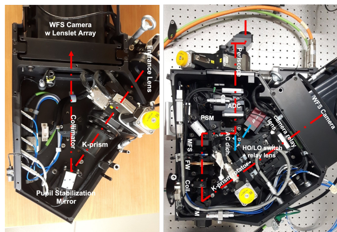
Figure 4. WFS view after removing cover. Left: LGS-WFS Right: NGS-WFS. See Ref. [9] for a detailed description of the components.
