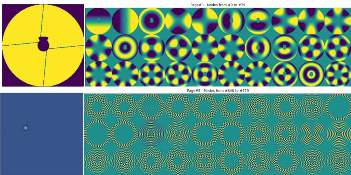
Figure 6. Top-left: pupil seen by ERIE, the asymmetry of the central obscuration is due to the M3 shadow in retracted position. Bottom-left: Example of Influence Function used to generate Karhunen-Loève basis. Right: subset of generated KL modes.
