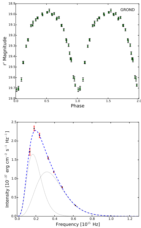
Fig. 2. Top to bottom: GROND light curve and spectrum of the 3FGL J0744.1-2523 candidate counterpart. The two BBs are shown as dotted lines.
