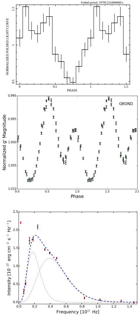
Fig. 1. Top to bottom: XMM-Newton light curve of the 3FGL J2039.6–5618 counterpart. GROND light curve and spectrum of its optical counterpart from GROND, UVOT, OM, and WISE data. The X-ray and optical light curve are aligned in phase. The dotted lines are the two BB components.
