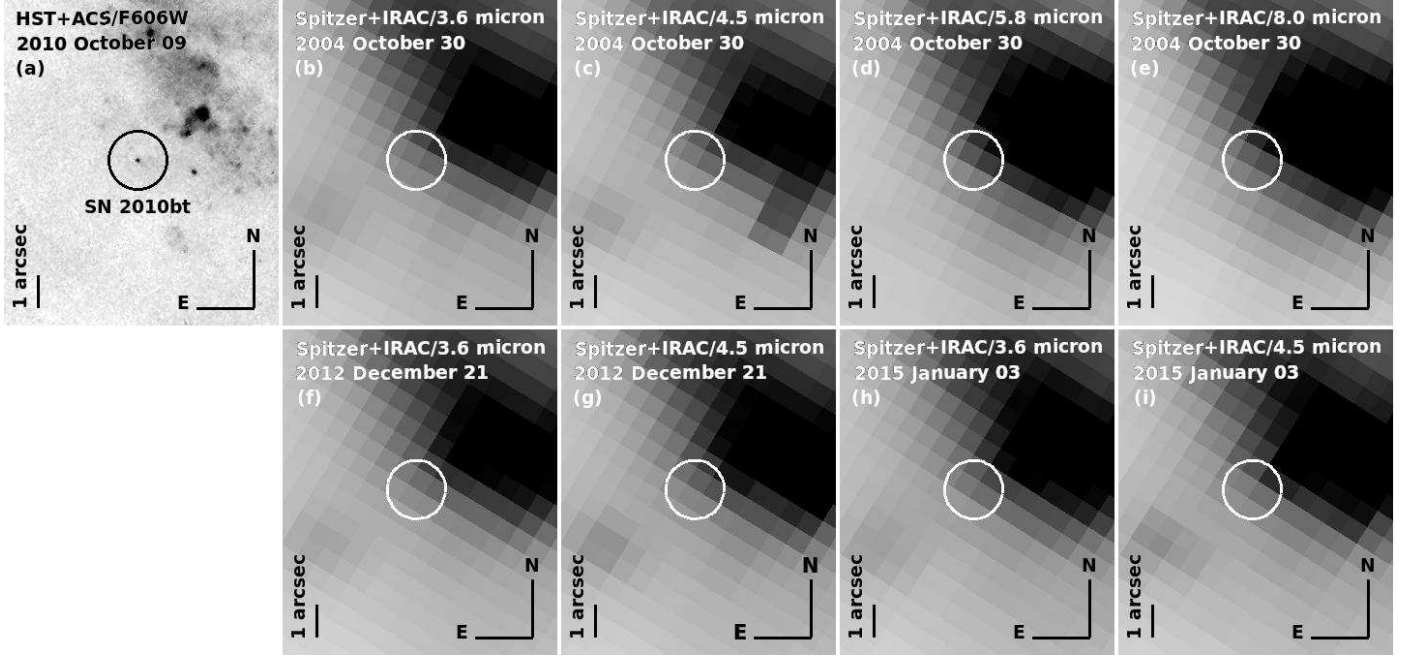
Figure 13. Subsections of (a) the post-explosion HST ACS/WFC image in F606W, along with (b–i) a sample of archival Spitzer images in different channels and epochs. The position of the SN is indicated by circles with a radius of 18 pixels ( 0.9'' ) for the HST image, and 1.5 pixels ( 0.9'' ) for the Spitzer images.
