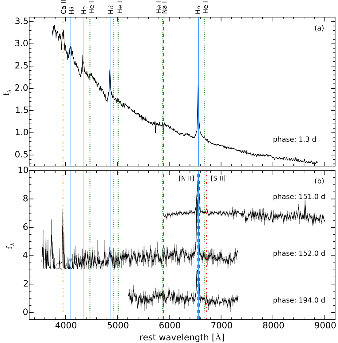
Figure 6. (a) Early-time and (b) late-time optical spectra of SN 2010bt. The late spectra are shown in grey, with a boxcar-smoothed (using a 5-pixel window) version of the spectra overplotted in black. The locations of the most prominent spectral features are indicated by vertical lines.
