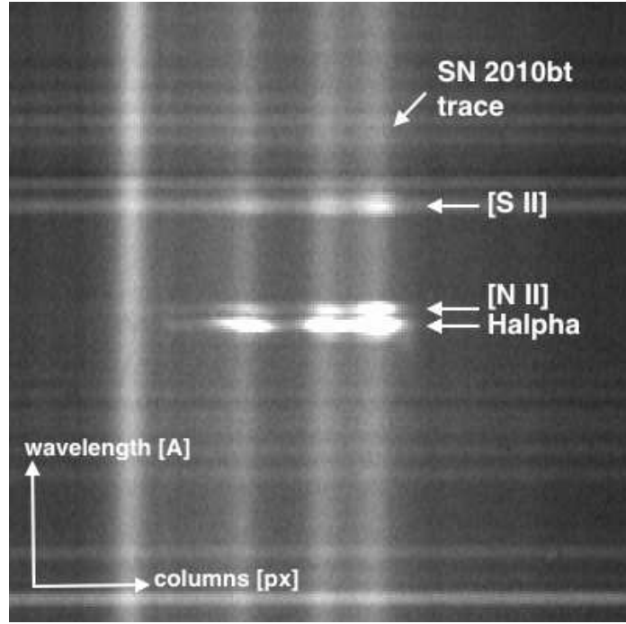
Figure 10. The H\alpha emission line in the 2D spectrum of SN 2010bt taken with NTT+EFOSC2 on 2010 September 15 (phase 161.0 d from the assumed V -maximum date).
