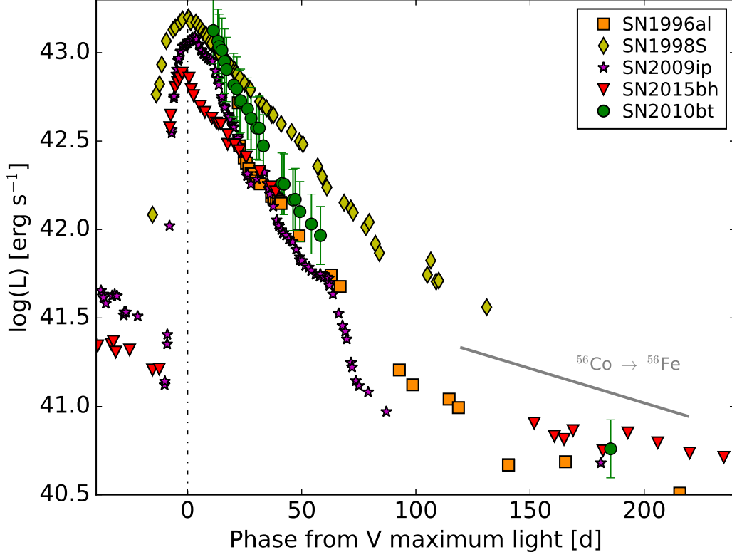
Figure 5. Pseudobolometric light curves of SN 2010bt ( circles ), compared with those of SNe 1996al ( squares ), 1998S ( diamonds ), 2009ip ( 5-pointed stars ), and 2015bh ( inverted triangles ). The dot-dashed vertical line indicates the V -band maximum light of SN 2010bt. Ages are relative to V maximum light (we have assumed V maximum date = discovery date − 10 d, for SN 2010bt).
