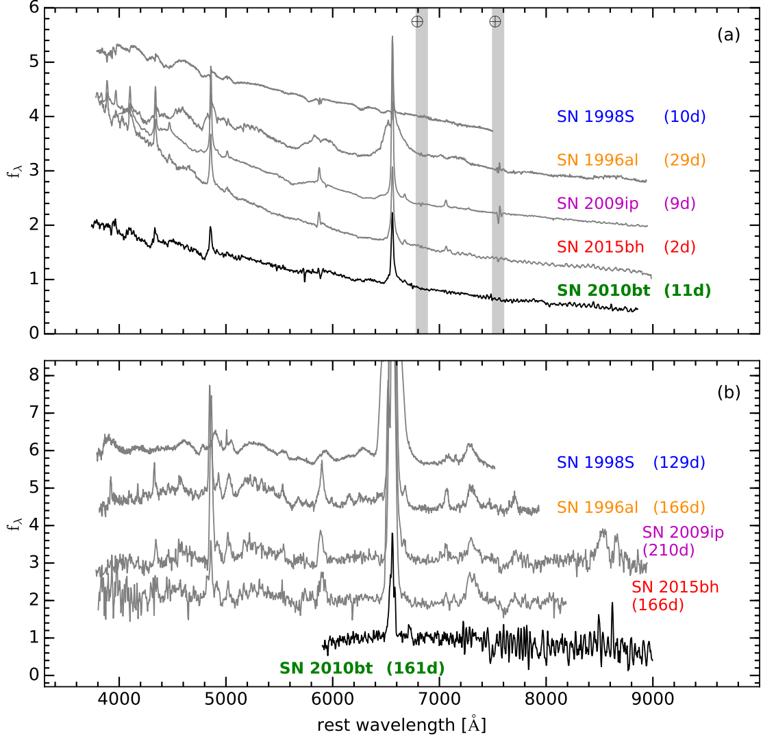
Figure 7. Comparison of SN 2010bt (a) early-time and (b) late-time optical spectra, along with those of the interacting SNe 1996al, 1998S, 2009ip, and 2015bh at similar epochs. All spectra have been corrected for their host-galaxy recession velocities and for extinction (values adopted from the literature; see also Table 6). Ages are relative to V maximum light.
