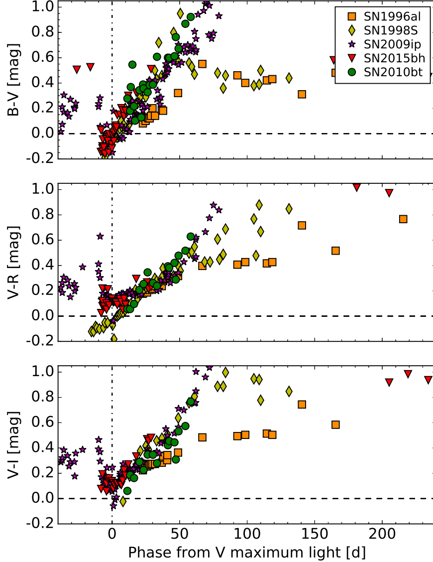
Figure 4. Intrinsic color curves of SN 2010bt ( circles ), compared with those of SNe 1996al ( squares ), 1998S ( diamonds ), 2009ip ( 5-pointed stars ), and 2015bh ( inverted triangles ). The dot-dashed vertical line indicates the V -band maximum light of SN 2010bt. Ages are relative to V maximum light (we have assumed V maximum date = discovery date -10 d, for SN 2010bt).
