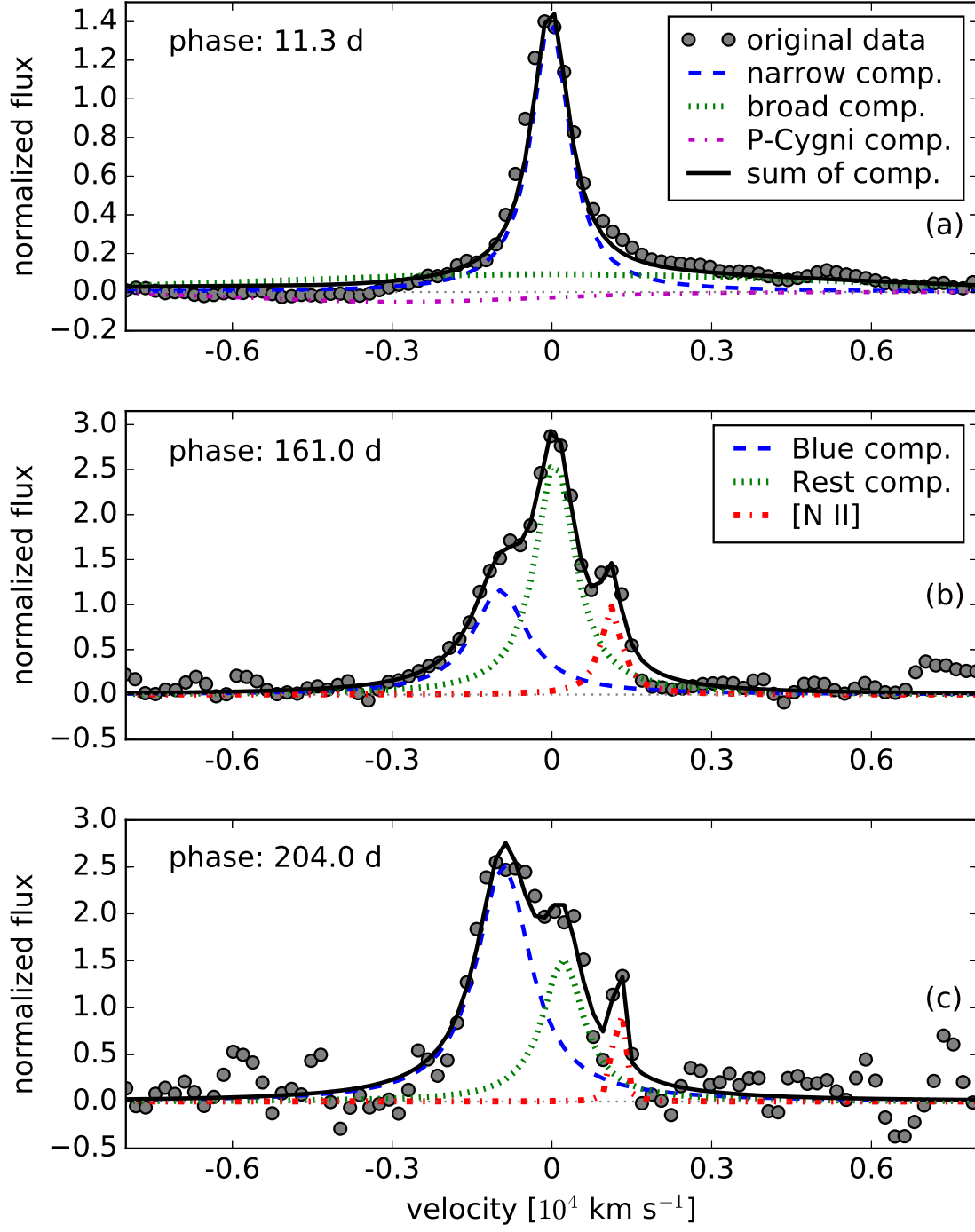
Figure 9. Decomposition of the H \alpha emission line of SN 2010bt at phases 11.3, 161.0, and 204.0 d from the assumed V -maximum date.
