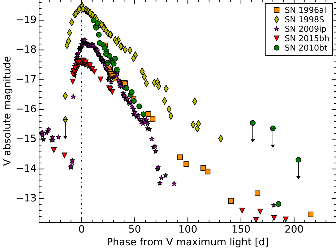
Figure 3. Absolute V light curve of SN 2010bt ( circles ) along with those of the SN IIn 1996al ( squares ), SN IIn 1998S ( diamonds ), the controversial transient SN 2009ip ( 5-pointed stars ), and SN 2015bh ( inverted triangles ). Upper limits are indicated by symbols with arrows. The dot-dashed vertical line indicates the V -band maximum light of SN 2010bt. Ages are relative to V maximum light (we have assumed V maximum date = discovery date -10 d, for SN 2010bt).
