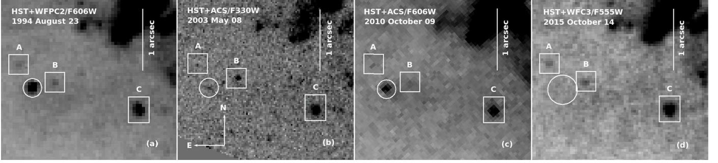
Figure 11. Subsections of the NGC 7130 pre-explosion (a) HST WFPC2 image in F606W and (b) HST ACS/HRC image in F330W, along with (c) the post-explosion HST ACS/WFC image of the SN site in F606W and (d) the late-time HST WFC3/UVIS image in F555W. The positions of the SN candidate progenitor and SN are indicated by circles , each with a radius of 3 pixels (between 0''.08 and 0''.15 ), except in panel (d), for which the radius is 6 pixels ( \sim 0''.23 ). The positions of three neighboring sources of SN 2010bt (“A,” “B,” and “C”) are also indicated.
