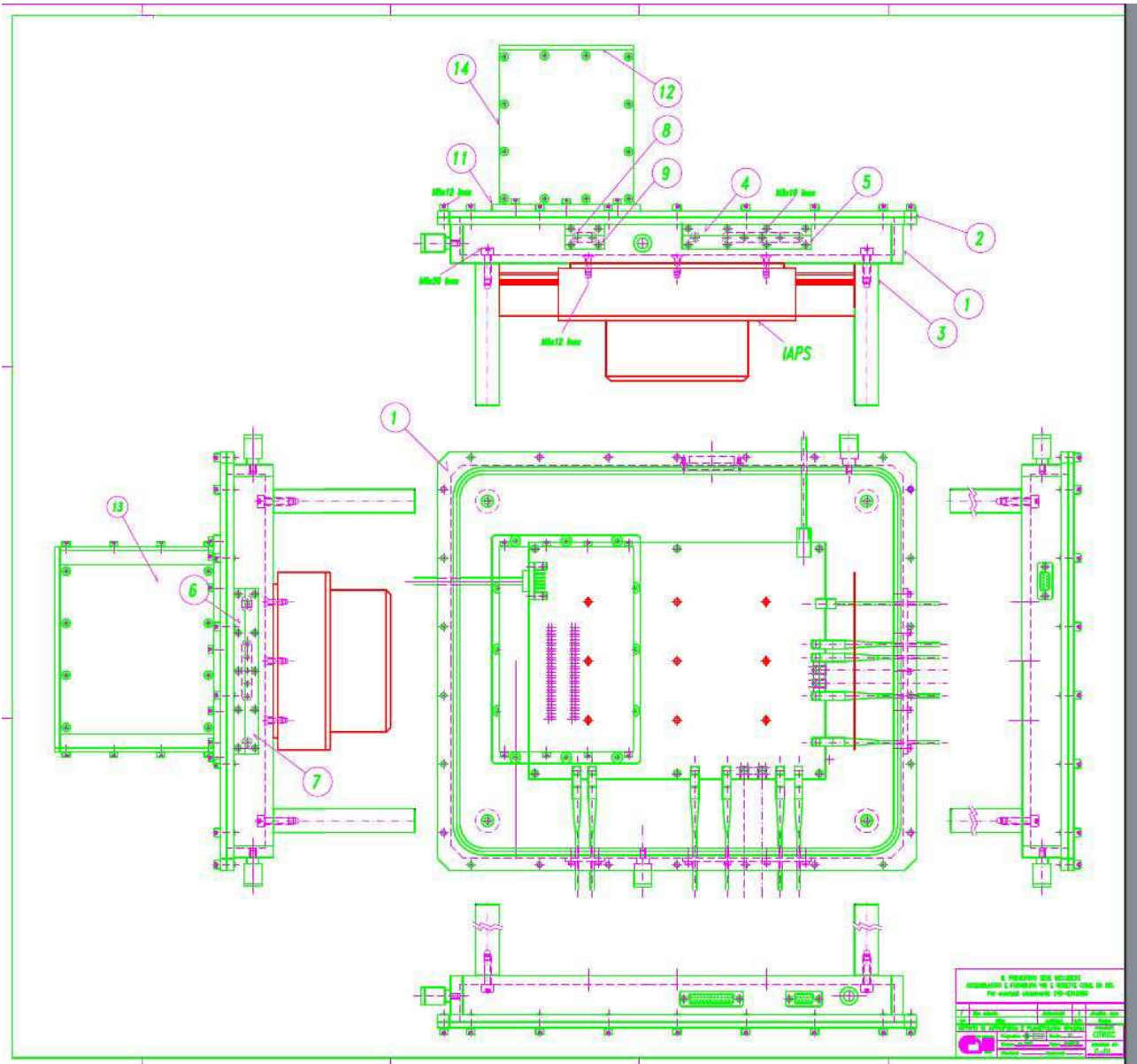
Figure 30: Custom designed box with Peltier assembly
