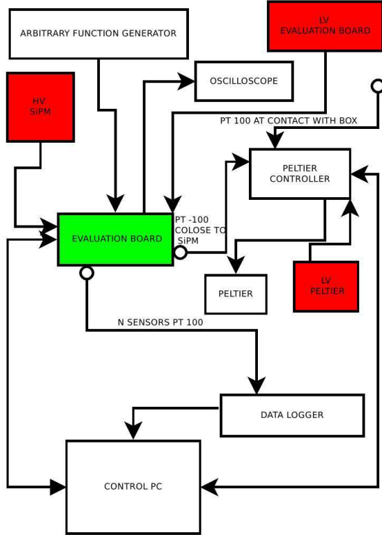
Figure 27: Block diagram of the experimental set-up
