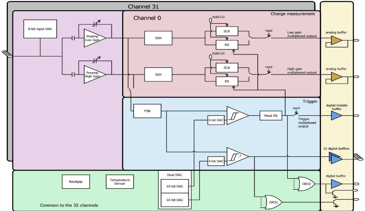
Figure 26: Architecture of the CITIROC ASIC
