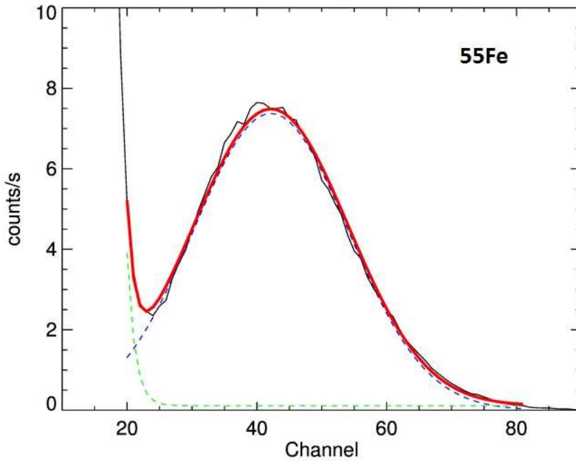
Figure 7: Spectrum of the 5.9 keV line of ^{55}\text{Fe} detected with the GAGG rod ( 3\text{ mm} \times 3\text{ mm} \times 30\text{ mm} ) and the LCT5 SiPM at the nominal overvoltage value of +3 V. The blue dashed line is the gaussian fit of the X-ray line, the green dashed line is the exponential fit of the dark current rate. The x axis does not start from 0 Channels.
