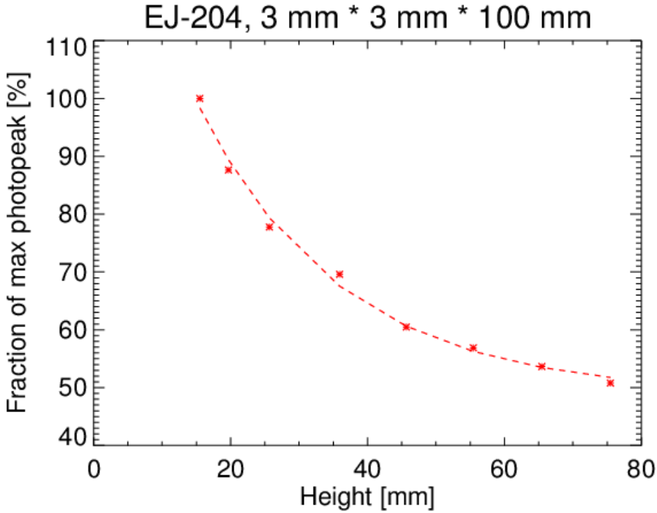
Figure 25: Fraction of the photopeak position as a function of height for a plastic scintillator rod of EJ-204 with 3\text{ mm} \times 3\text{ mm} \times 10\text{ cm} size. The height is measured from the PMT entrance window. The minimum height is 15 mm and is due to the experimental set-up.
