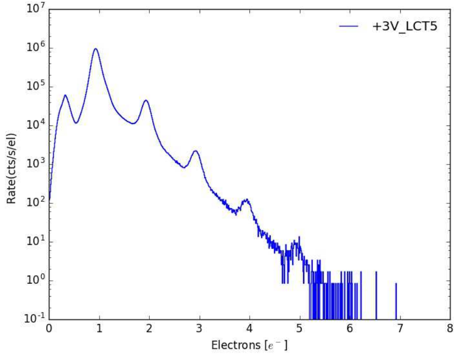
Figure 16: Spectrum of the dark current rate at room temperature ( \sim 22 - 25 °C) from an LCT5 SiPM with pitch of 50 \mu\text{m} and overvoltage of +3 V.
