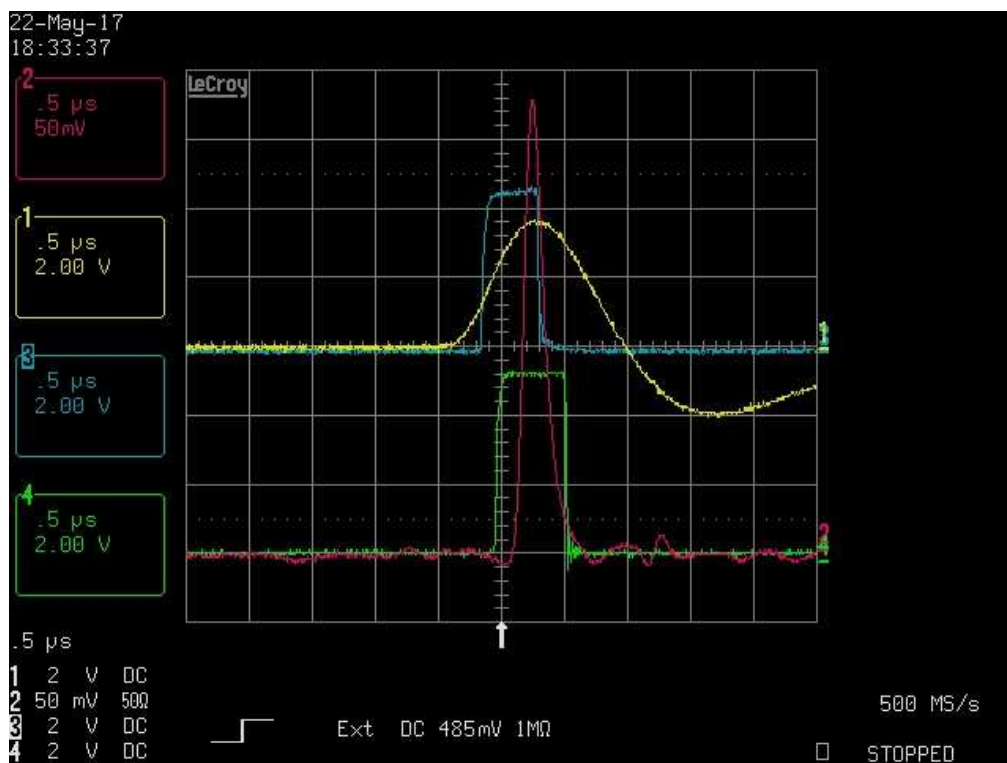
Figure 24: Oscilloscope screenshot with the following signals: CH1 (yellow): output from Ortec 4890 (Brillance 380) after delay of 0.5 \mu s; CH2 (magenta): Ortec 474 (SiPM) after delay of 1.25 \mu s; CH3 (cyan): SCA of Ortec 4890 (Brillance 380); CH4 (green): SCA of Ortec 850 (SiPM);
