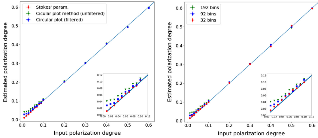
Fig. 7. Left panel: comparison between polarization estimated obtained by means of the Stokes' parameters (filled circles) vs the circular plot method (unfiltered: downward triangles, filtered: filled squared points). Right panel: the comparison between polarization estimated obtained by applying the unfiltered circular correlation method with a different binning of the modulation histograms. The green downward triangles in two panels refer to the same data (unfiltered circular correlation method) applied to a modulation histogram with 192 bins.
