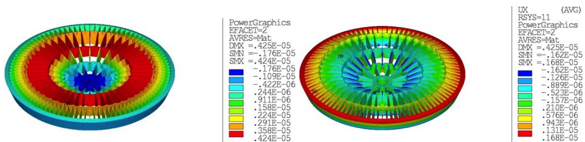
Figure 4: Axial displacements (Left) and radial displacements (Right) at gravity release. The range of spoke wheel displacement components is -1.8 / +4.2 \mu\text{m} axial -1.6 / +1.7 \mu\text{m} radial.
