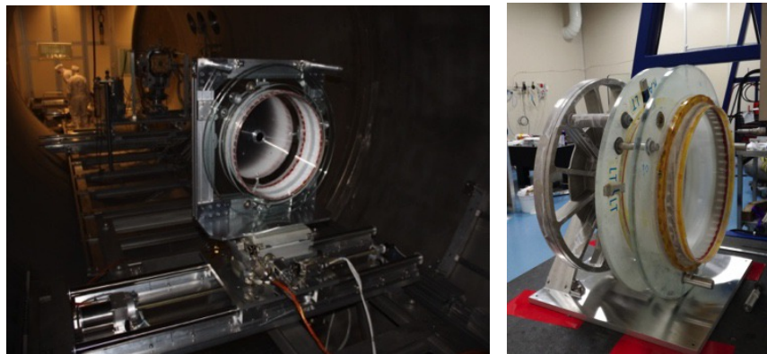
Figure 15: (Left) The jig used to support the SSS with the shell#7 during the measurements @Panter in 2011. (Right) The Invar Spoke Wheel (ISW), added to the SSS during the manufacturing of the Shell#4, is interfaced to the new jig for calibration.
