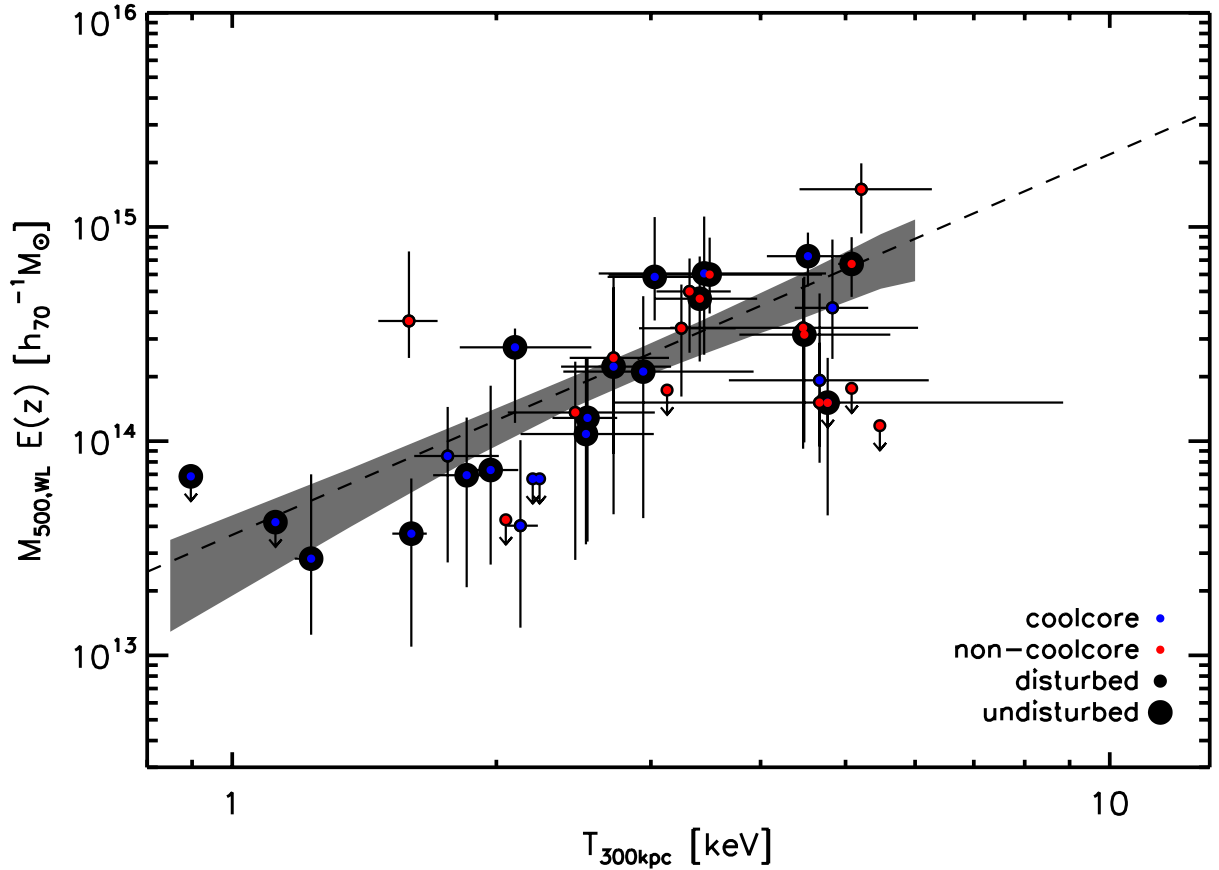
Fig. 4. Mass-temperature relation for 38 clusters drawn from XXL-100-GC for which weak-shear information is available from CFHTLenS. The line is the highest posterior density fit and the shaded region is the credible region. Systems with upper limits on mass are indicated by arrows and plotted at 3\sigma confidence.
