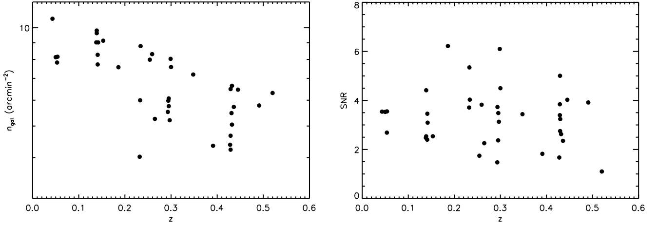
Fig. 3. Left: number density of background galaxies behind each galaxy cluster versus cluster redshift. Right: weak-lensing shear signal-to-noise ratio as a function of cluster redshift.
