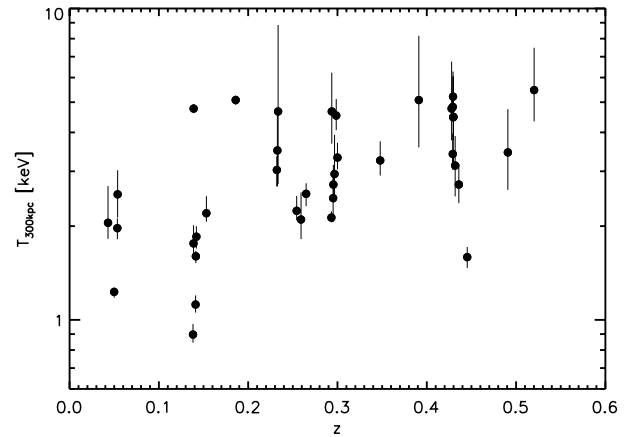
Fig. 2. Redshift versus X-ray temperature T_{300\text{kpc}} for the 38 clusters from XXL-100-GC that are located within the CFHTLenS shear catalogue footprint.
