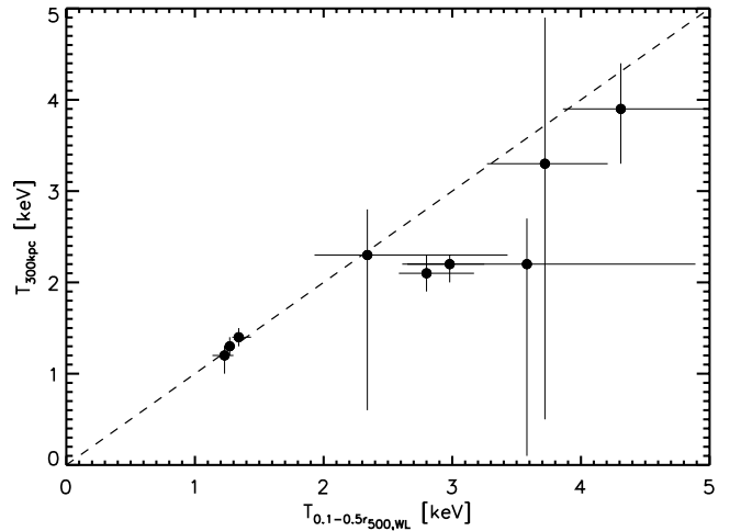
Fig. 7. Comparison of core excised X-ray temperatures (Kettula et al. 2013) and the re-derived temperatures measured within a 0.3 Mpc aperture. The dashed line is equality.
