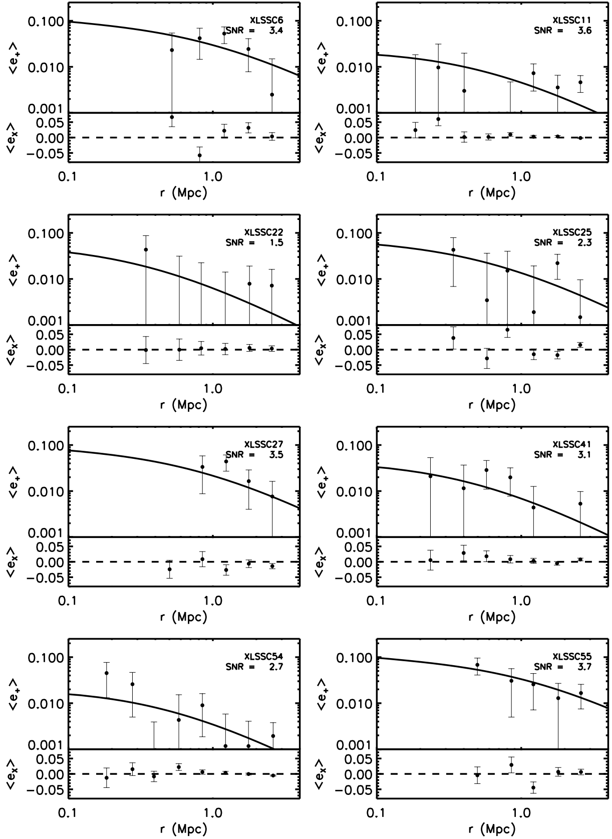
Fig. A.1. Tangential and cross-component ellipticity as a function of distance from cluster centre.
