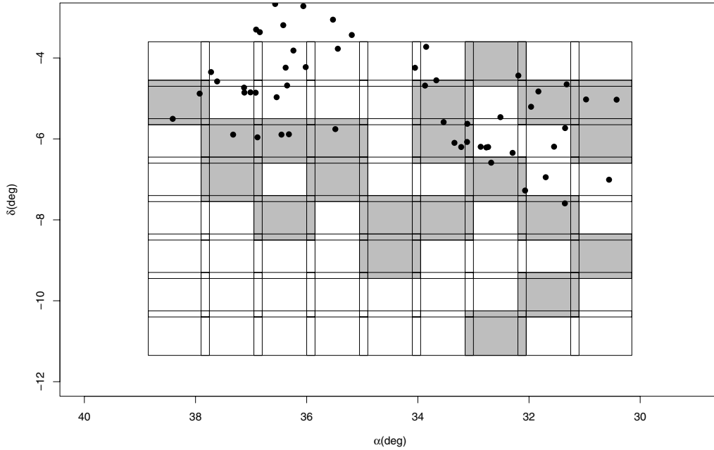
Fig. 1. Overlap of XXL-100-GC with the CFHTLenS W1 field. The boxes are individual pointings in CFHTT with XXL-North field clusters (filled points). The shaded boxes are pointings that fail the CFHTLenS weak-lensing field selection criteria (see Sect. 4.1).
