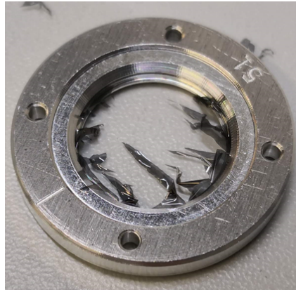
Fig. 67 - LAOF-CNT2-C1B2-F01 filter damaged during manipulation.
