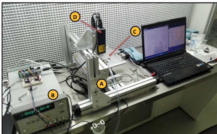
Fig. 78 – Set-up to measure the deformation and resistance of filter samples under static differential pressure. A) Motorized X-Y-Z table, B) Power supply, microcontroller and stepper motor drivers, C) Pressure chamber, D) Distance sensor.
