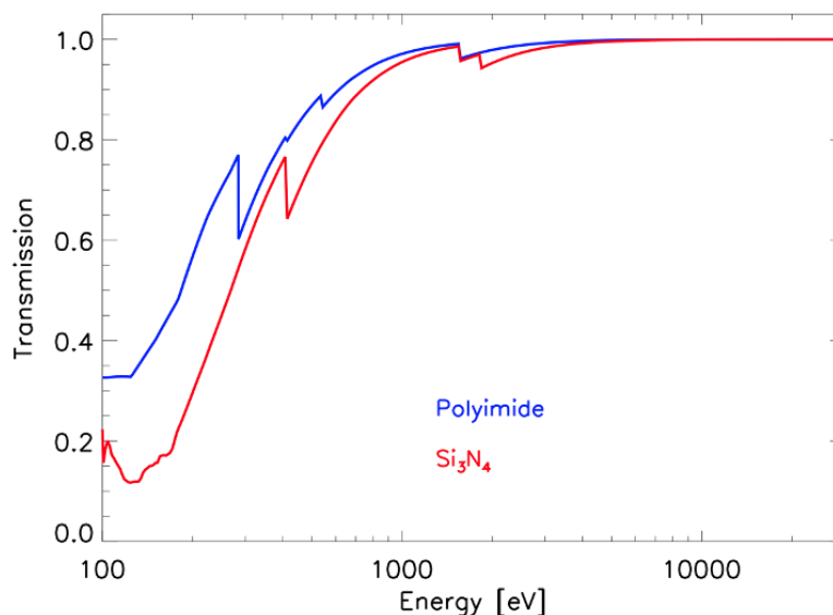
Fig. 81 - X-ray modelled transmission for two filters of Polyimide and \text{Si}_3\text{N}_4 both 50 nm thick coated with 30 nm of aluminum.
