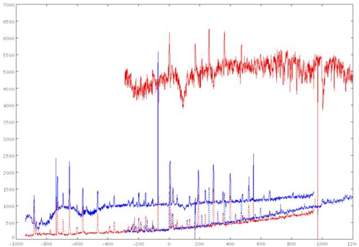
Figure 4: blue solid line: start extracted from 0152 (raw), slit 3 blue dot line sky extracted from 0152 (raw), list 11 red solid line star extracted from 0134 (raw), slit 11 red dot line sky extracted from 0134 (raw), slit 3
