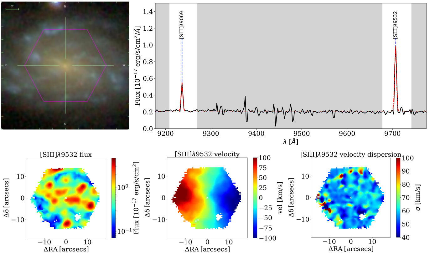
Fig. 1. Top left: g-r-i image composite from SDSS for MaNGA galaxy 8150-6103, with the MaNGA IFU hexagonal FoV overlaid. East is to the left. Top right: An example of our fitting procedure for the [S III] lines for one representative spaxel in this example galaxy. The black solid line is the observed spectrum, while the dashed-dotted red line is the best-fit. The regions in grey were masked before fitting. Bottom panels: [S III] 9532 flux, velocity and velocity dispersion maps of MaNGA galaxy 8150-6103.
