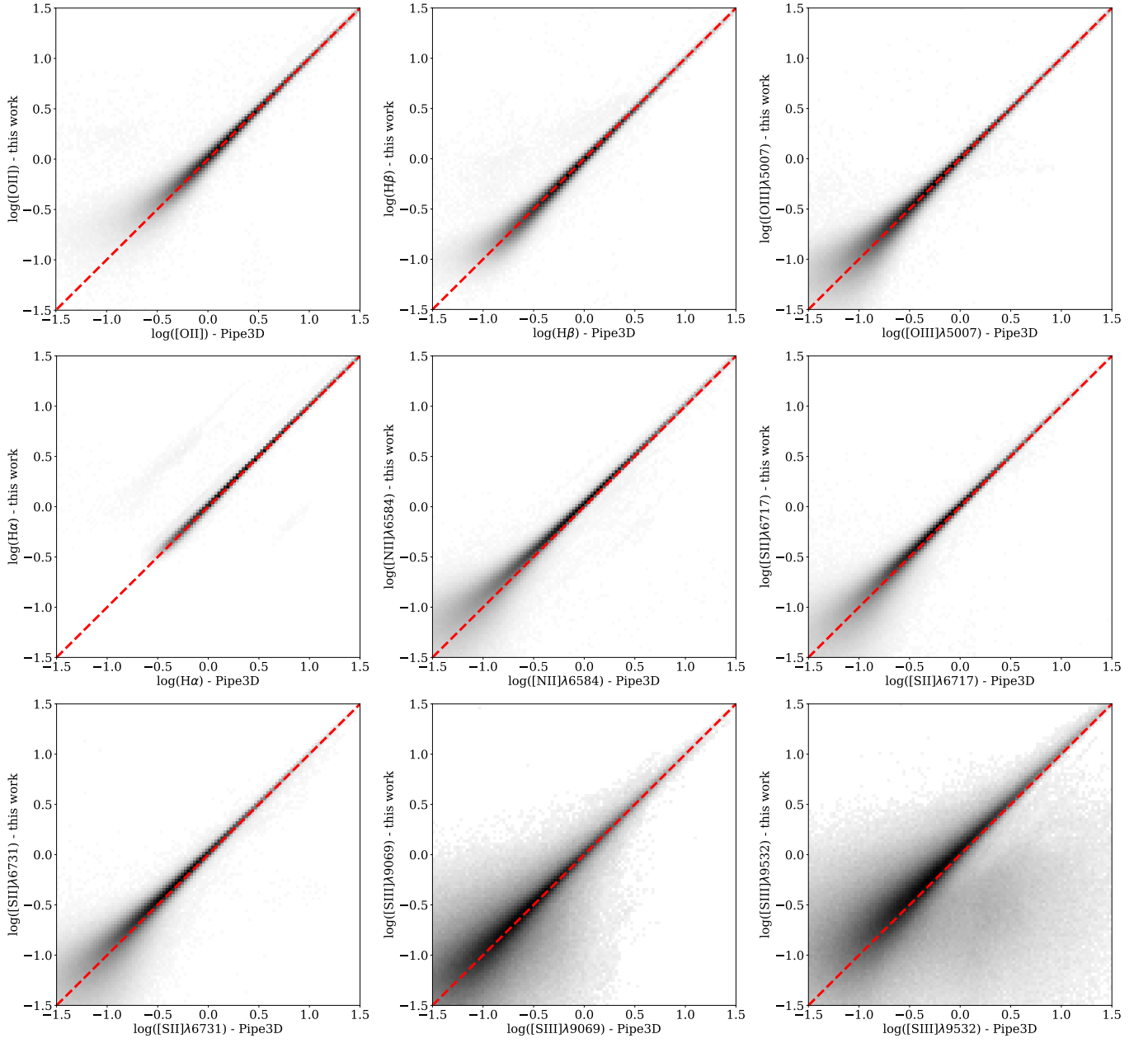
Fig. A.1. Spaxel-by-spaxel comparison between the emission line fluxes taken into account in this work (y-axis) and the results of Pipe3D (x-axis): namely [O II], H \beta , [O III] \lambda 5007, H \alpha , [N II] \lambda 6584, [S II] \lambda 6717, [S II] \lambda 6731, [S III] \lambda 9069, [S III] \lambda 9532. The fluxes are in units of 10^{-17} erg s ^{-1} Å ^{-1} cm ^{-2} and are expressed in logarithm. The red dashed line represents the one-to-one line.
