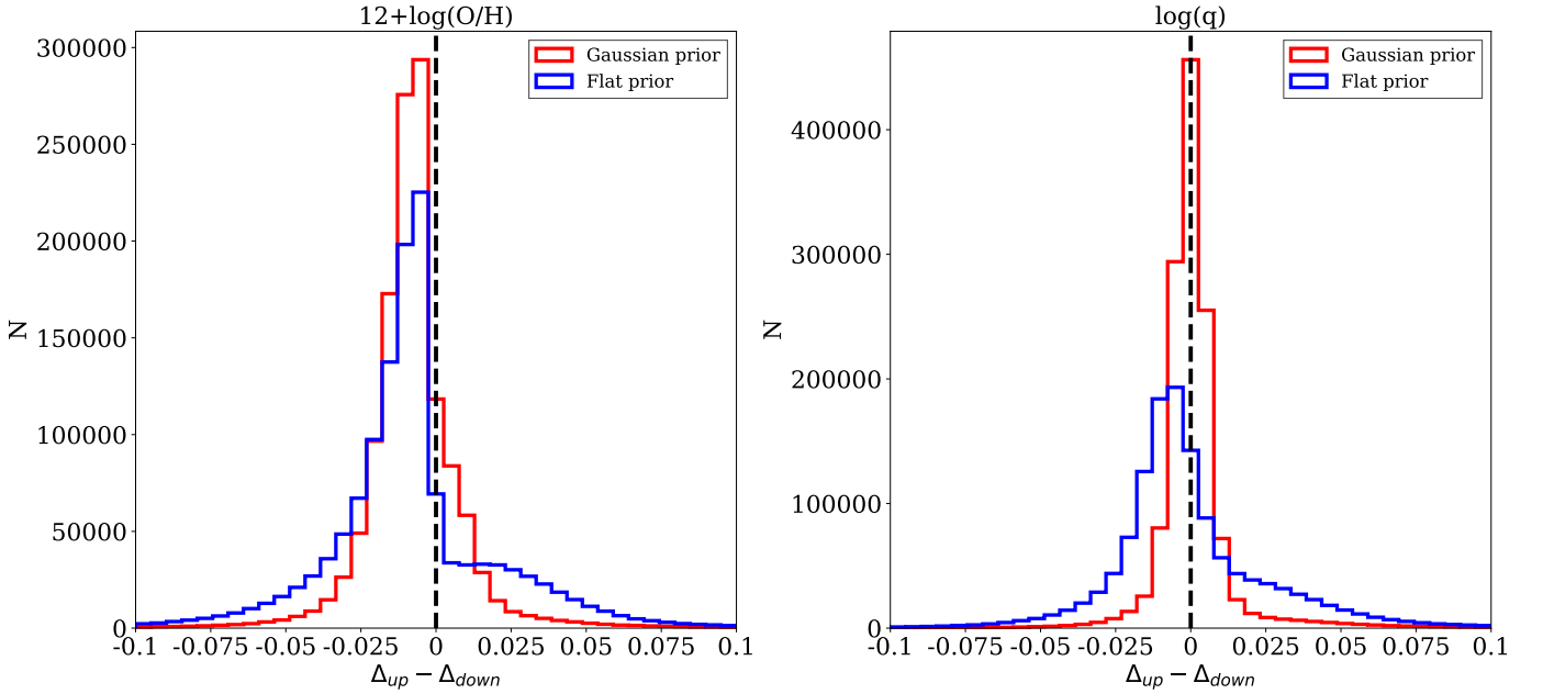
Fig. 8. Distribution of the difference between \Delta_{up} = 84^{th} - 50^{th} and \Delta_{down} = 50^{th} - 16^{th} for the metallicity (left panel) and ionisation parameter (right panel), in the case with a flat (in blue) and a Gaussian (in red) prior on the ionisation parameter, respectively, for all the spaxels of all the galaxies.
