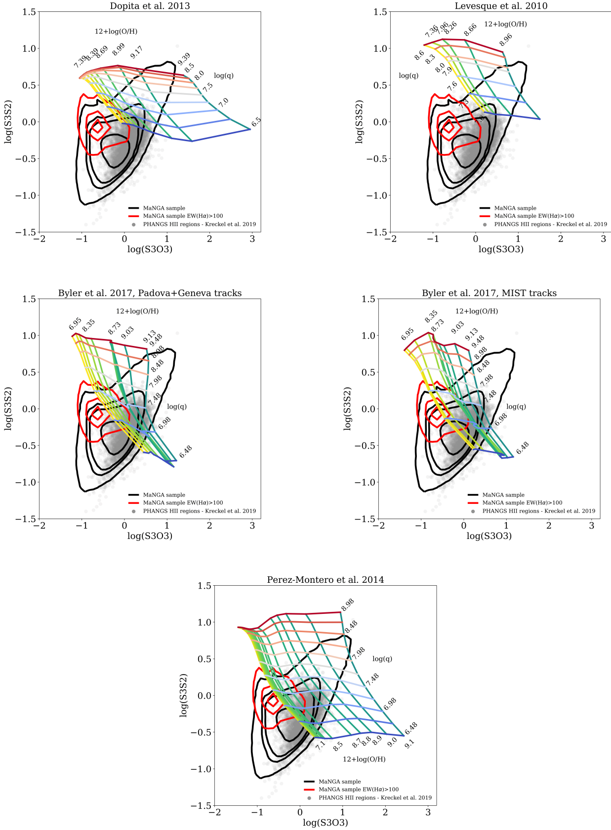
Fig. 3. [S\text{ III}]/[O\text{ III}] versus [S\text{ III}]/[S\text{ II}] diagnostic diagrams introduced by Stasińska (2006) showing the density contours for all the star-forming spaxels of our sample (in black), with superimposed Dopita et al. (2013), Levesque et al. (2010), Byler et al. (2017) pdva+geneva, Byler et al. (2017) MIST, and Pérez-Montero (2014) models respectively. Metallicity increases horizontally from yellow to green, while ionisation parameter increases vertically [redder means higher \log(q) and bluer lower \log(q) ]. The red contours correspond to the brightest MaNGA star-forming regions [ EW(H\alpha) > 100 ], while the grey dots are the H II regions analysed by Kreckel et al. (2019) with the PHANGS survey. Current photoionisation models fail to reproduce the observed [S\text{ III}] lines.
