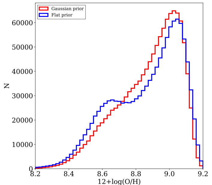
Fig. 4. Distribution of the best-fit values of 12+\log(O/H) for all MaNGA spaxels considered in this work. Metallicities are derived by IZI with a Gaussian (red) and a flat (blue) prior on the ionisation parameter, respectively. Specifically, the mean of the Gaussian prior is given by the Diaz et al. (1991) calibration, that links [S III]/[S II] line and ionisation parameter.
