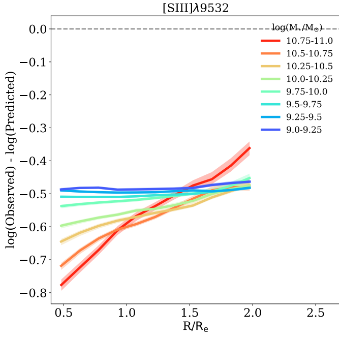
Fig. C.2. Radial distribution of the difference between the logarithm of the observed [\text{S III}]\lambda 9532 flux and that of the best-fit model (both normalised to \text{H}\beta ) predicted by IZI, in eight stellar mass M_* bins, as reported in the legend. This clearly shows that [\text{S III}]\lambda 9532 is largely overestimated, with differences between observed and predicted fluxes up to 0.8 dex.
