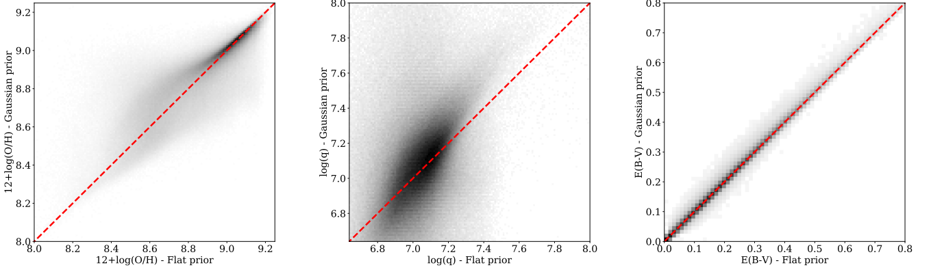
Fig. 7. Comparison between the results obtained with IZI with a flat (x-axis) and a Gaussian (y-axis) prior on the ionisation parameter, for metallicity, ionisation parameter and gas extinction, respectively. The red dashed line represents the one-to-one relation.
