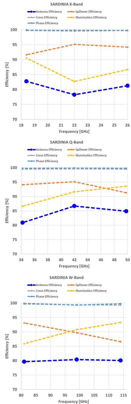
Figure 3. Aperture efficiency and individual efficiency terms for the tri-band receiver of the SRT.
