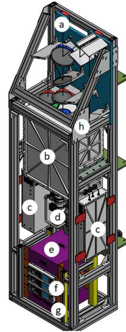
Figure 1. 3D drawing of the receiver for SRT. The main elements are the following ones: (a) Quasi-optics system; (b) Cryogenic feed system; (c) Warm RF/IF sections; (d) Pump & CTI-350; (e) M&C unit (provided by INAF); (f) Synthesizers; (g) Power supplier; (h) Anchoring system.
