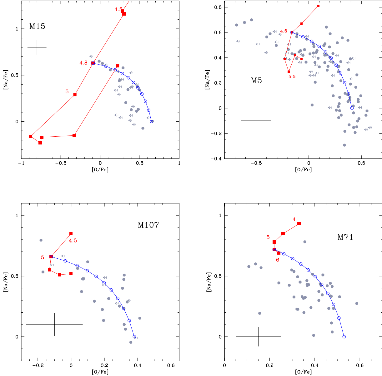
Figure 11. Dataset from Carretta et al. (2009a,b) in the O-Na plane are shown in gray for M15 (top-left), M5 (top-right), M107 (bottom-left) and M71 (bottom-right). Upper limits in O abundances are shown as arrows, detections are indicated as circles. AGB yields (red squares) and their corresponding dilution curves (blue open circles) are also shown according to the metallicity of each cluster.
