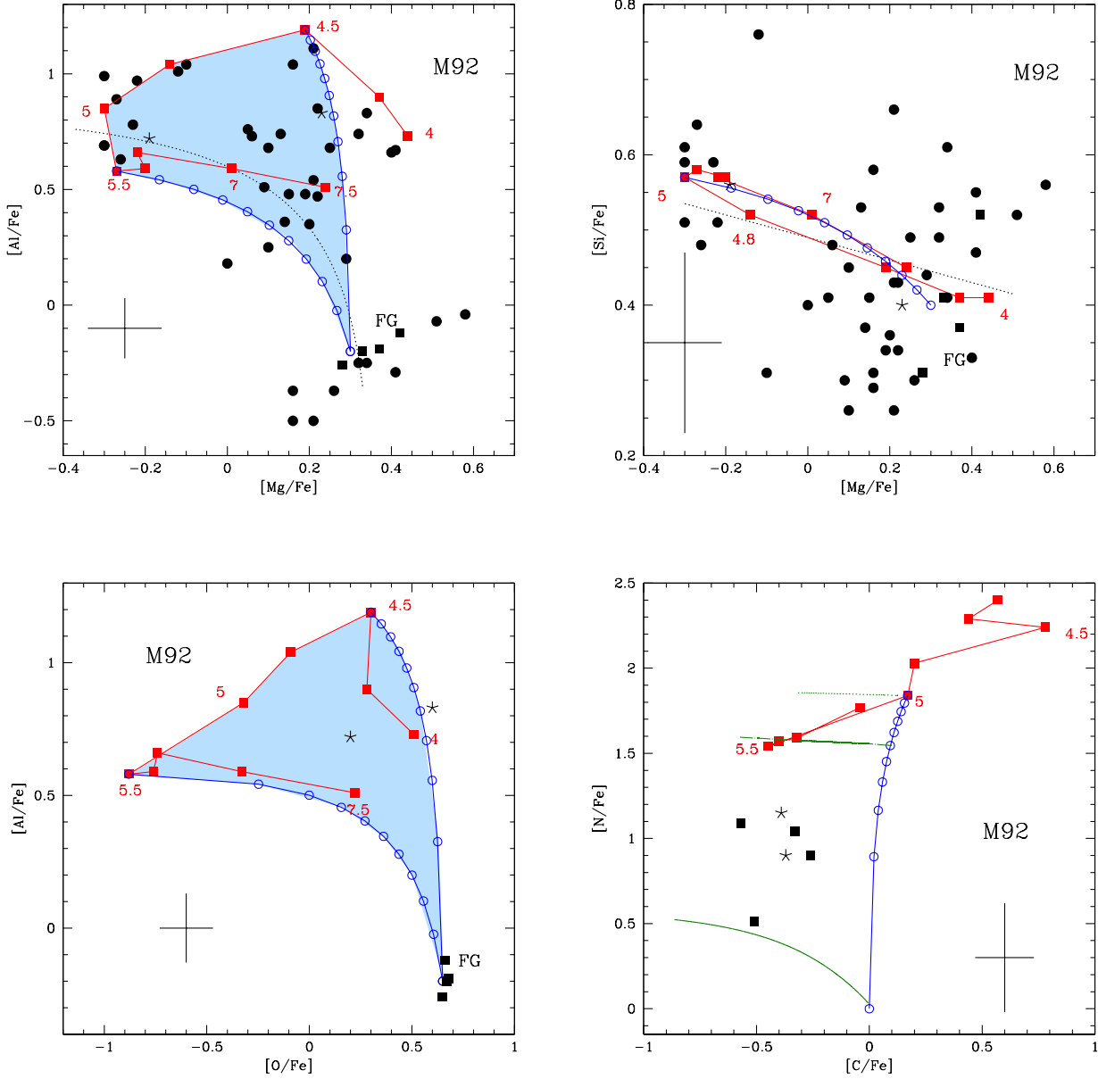
Figure 3. M92 stars from ME15 are shown in the same planes and with the same symbols as in Figure 2. They are compared with the yields of AGB models of the same metallicity ( Z = 2 \times 10^{-4} ) as in the case of M15.
