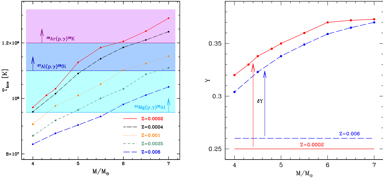
Figure 1. Left: typical temperature at the base of the convective envelope during the AGB phase, as function of the initial mass of the star at different metallicities. The temperatures above which some important nuclear reactions (labelled) are efficient are shown as horizontal lines and correspondent shaded area. Right: helium yields as function of stellar masses for the highest ( Z = 6 \times 10^{-3} , solid-red line) and lowest ( Z = 2 \times 10^{-4} , dashed-blue line) metallicity considered in this work. The horizontal lines at Y=0.26 and Y=0.25 represent the initial helium content considered respectively.
