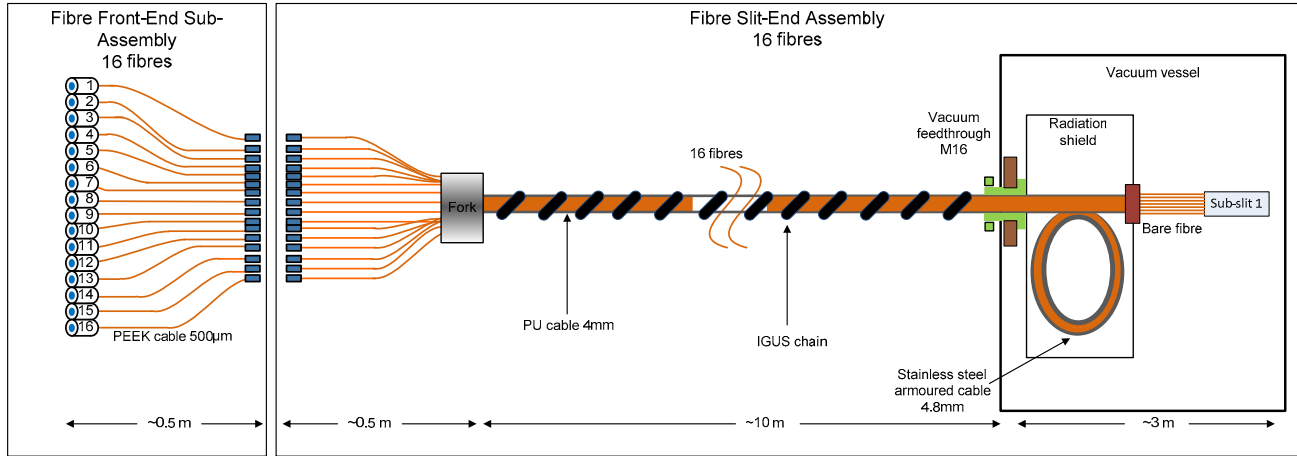
Figure 1 Bundle design
