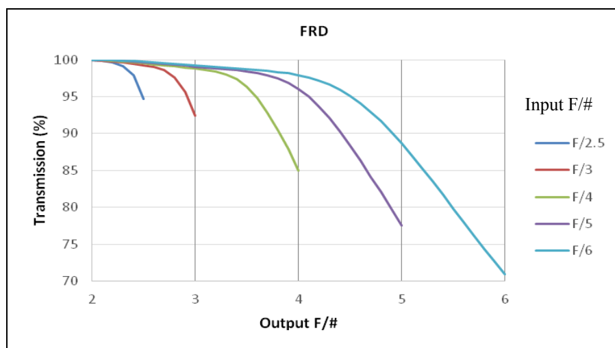
Figure 13 FRD curves of bare fibre
