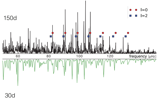
FIGURE 6 Power spectral density as a function of frequency obtained by considering time series of duration 150 and 30 days for a bright ( m_V = 9 ) giant observed by Kepler . The individual mode frequencies of radial ( l = 0 ) and quadrupolar modes ( l = 2 ) are indicated in the upper panel by red circles and blue squares, respectively. In the 30-days-long time series, the robust identification of individual mode frequencies is hindered by the low frequency resolution, leading to a much reduced precision and accuracy on the inferred properties of the individual modes
